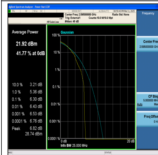
Band38-5MHz-64QAM-38000-1RB#0-PASS
