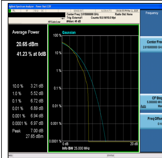
Band38-10MHz-64QAM-38200-1RB#0-PASS
