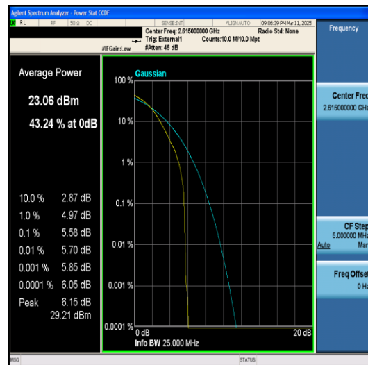
Band38-10MHz-QPSK-38200-50RB#0-PASS
