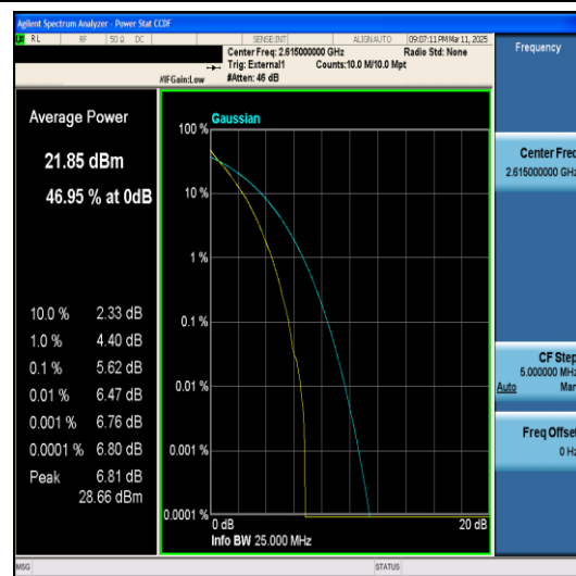
Band38-10MHz-QPSK-38200-50RB#0-PASS
