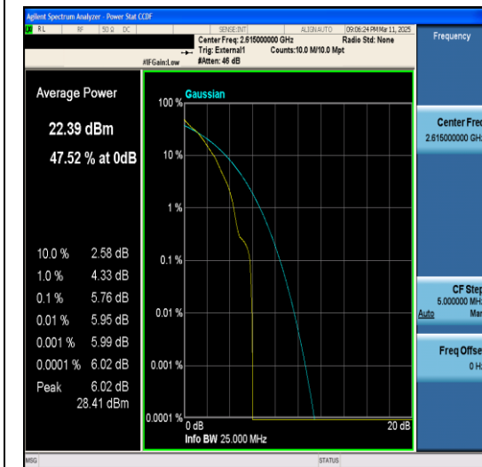
Band38-10MHz-64QAM-38200-1RB#0-PASS
