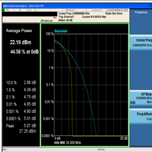
Band38-20MHz-QPSK-38000-100RB#0-PASS
