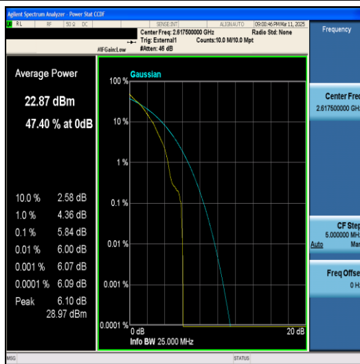
Band38-5MHz-64QAM-38225-1RB#0-PASS
