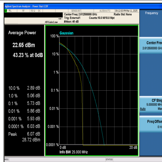
Band38-15MHz-QPSK-38175-75RB#0-PASS
