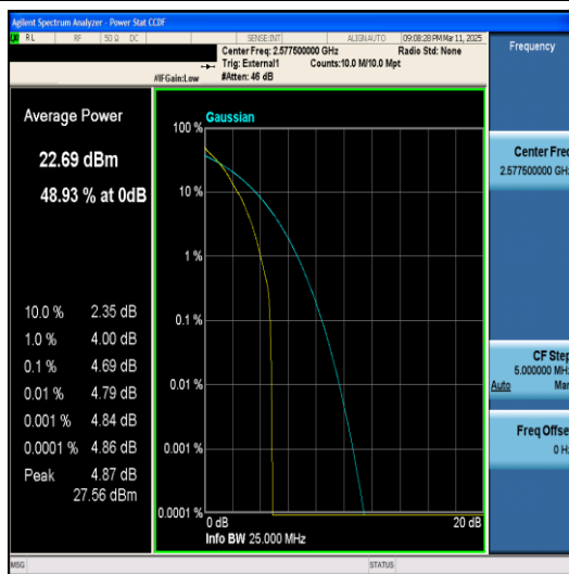
Band38-15MHz-64QAM-37825-1RB#0-PASS
