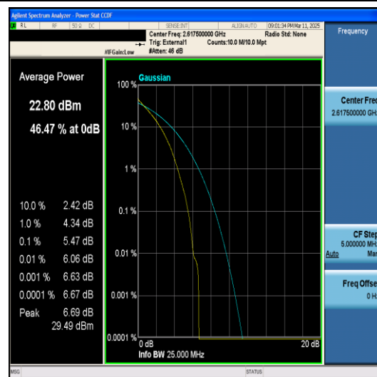
Band38-5MHz-QPSK-38225-25RB#0-PASS
