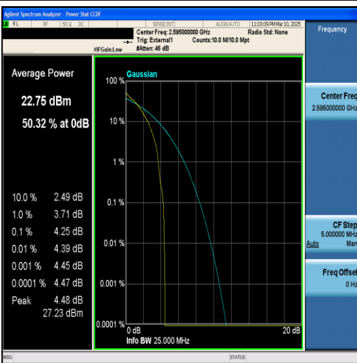
Band38-20MHz-64QAM-38000-1RB#0-PASS
