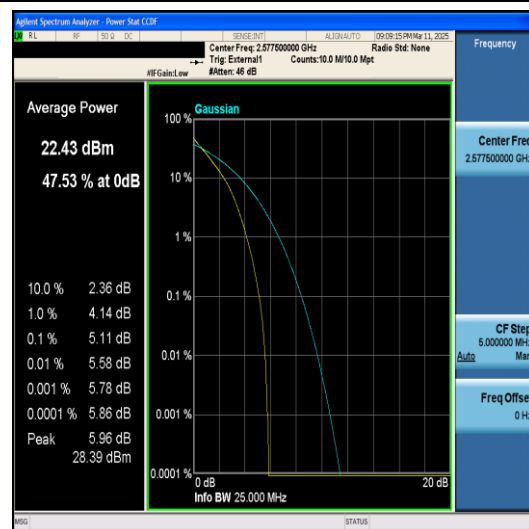
Band38-15MHz-QPSK-37825-75RB#0-PASS
