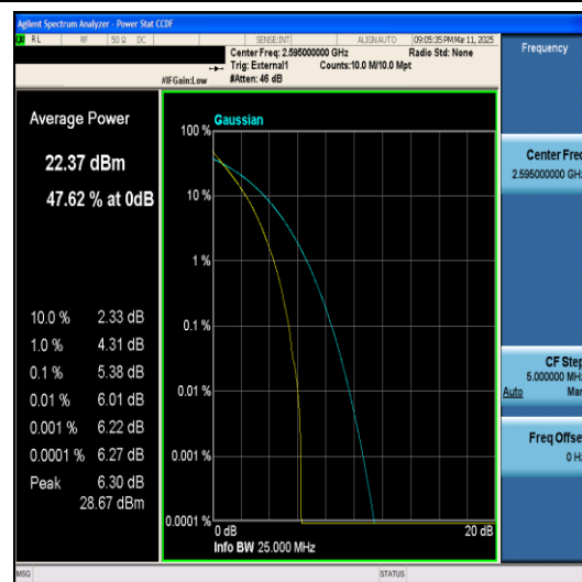
Band38-10MHz-QPSK-38000-50RB#0-PASS
