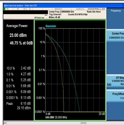
Band38-5MHz-QPSK-38000-25RB#0-PASS
