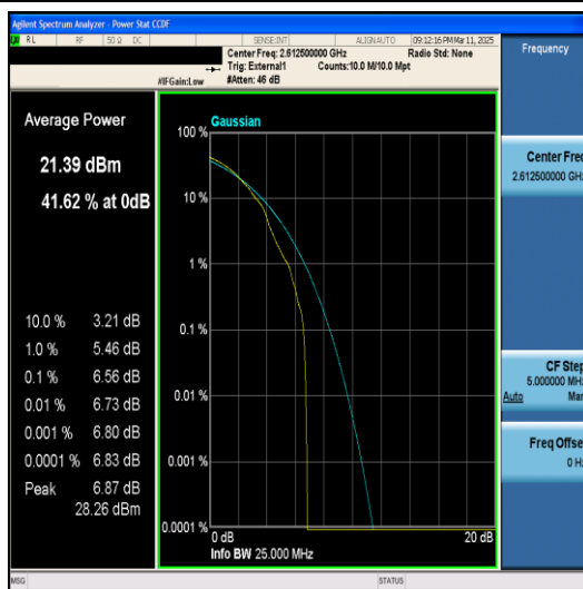
Band38-15MHz-64QAM-38175-1RB#0-PASS
