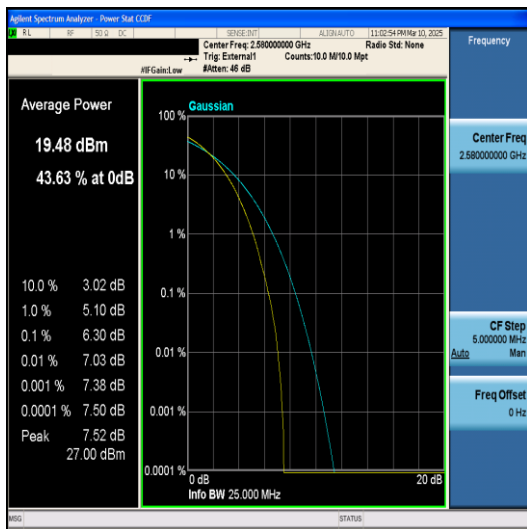
Band38-20MHz-16QAM-38000-1RB#0-PASS
