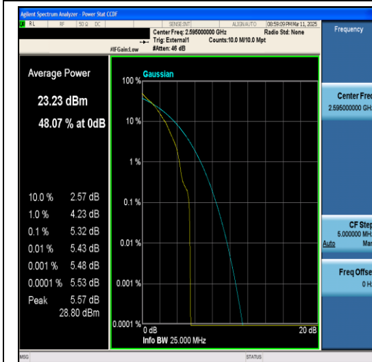
Band38-5MHz-64QAM-38000-1RB#0-PASS
