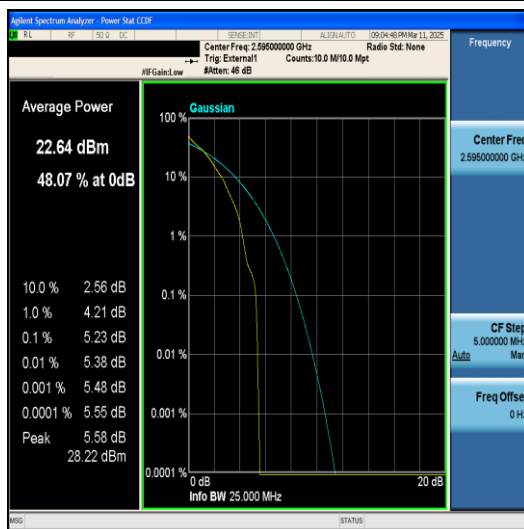
Band38-10MHz-64QAM-38000-1RB#0-PASS
