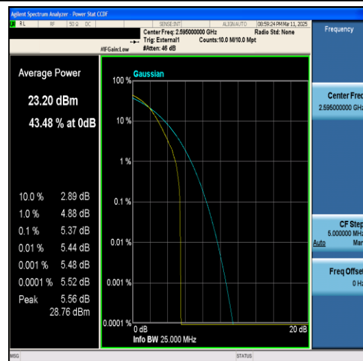
Band38-5MHz-QPSK-38000-25RB#0-PASS
