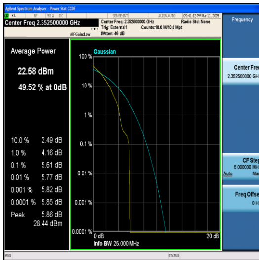
Band40(2345-2360)-5MHz-QPSK-39175-1RB#0-P
