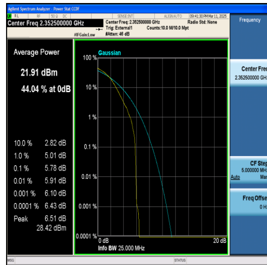
Band40(2345-2360)-5MHz-16QAM-39175-1RB#0-
