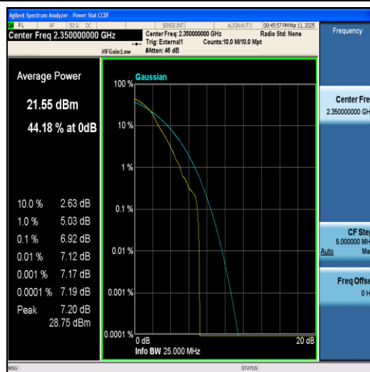
Band40(2345-2360)-10MHz-16QAM-39150-1RB#
