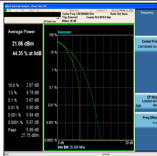
Band41-10MHz-QPSK-39700-50RB#0-PASS
