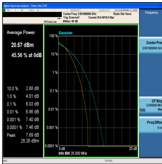
Band41-10MHz-QPSK-40620-1RB#0-PASS
