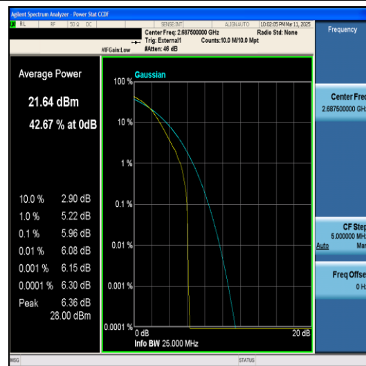
Band41-5MHz-QPSK-41565-25RB#0-PASS
