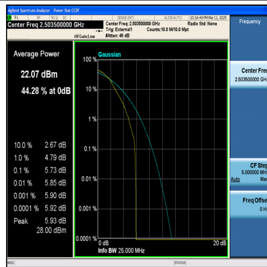
Band41-15MHz-QPSK-39725-75RB#0-PASS
