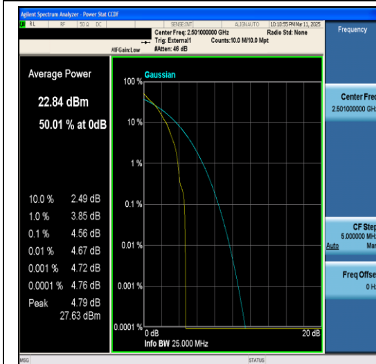
Band41-10MHz-64QAM-39700-1RB#0-PASS
