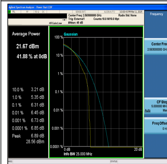
Band41-5MHz-64QAM-40620-1RB#0-PASS
