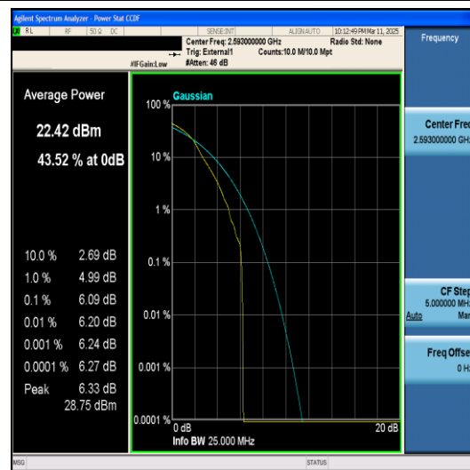
Band41-10MHz-QPSK-40620-50RB#0-PASS
