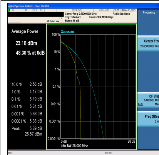
Band41-5MHz-64QAM-40620-1RB#0-PASS
