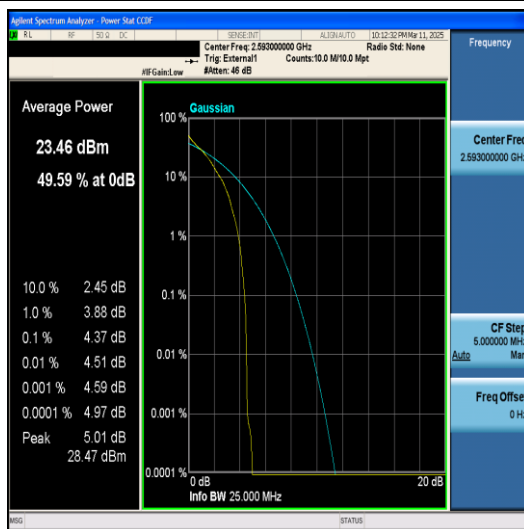
Band41-10MHz-64QAM-40620-1RB#0-PASS
