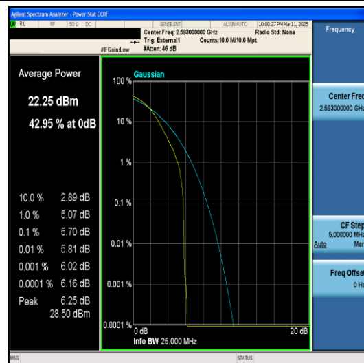
Band41-5MHz-QPSK-40620-25RB#0-PASS
