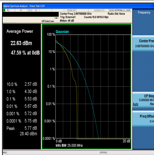
Band41-5MHz-64QAM-41565-1RB#0-PASS
