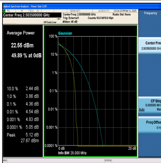
Band41-15MHz-64QAM-39725-1RB#0-PASS
