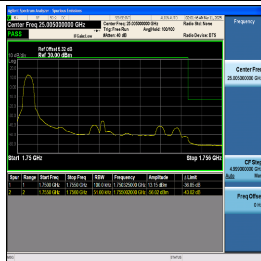
Band4-5MHz-QPSK-20375-1RB#0-PASS
