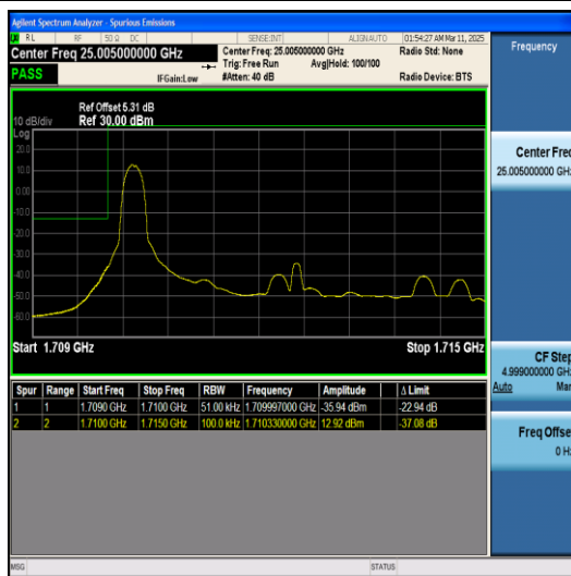
Band4-5MHz-QPSK-19975-25RB#0-PASS
