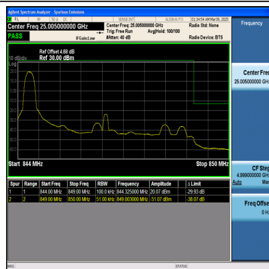
Band5-5MHz-QPSK-20625-1RB#0-PASS
