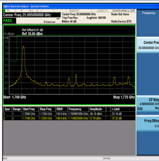
Band4-15MHz-QPSK-20025-75RB#0-PASS
