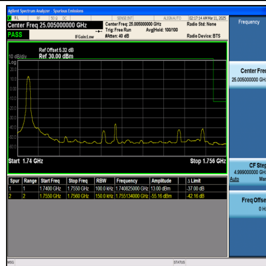
Band4-15MHz-QPSK-20325-1RB#0-PASS
