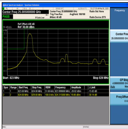
Band5-5MHz-QPSK-20425-25RB#0-PASS
