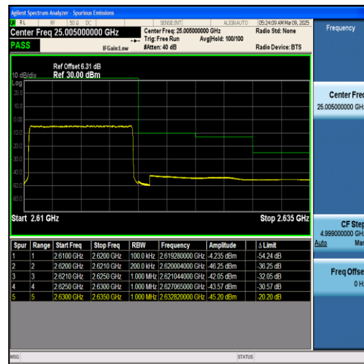
Band38-15MHz-QPSK-37825-1RB#74-PASS
