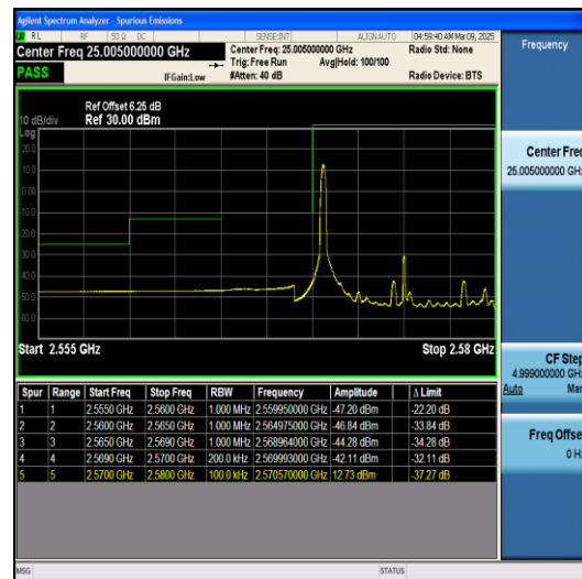
Band38-10MHz-QPSK-37800-50RB#0-PASS
