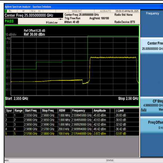
Band38-10MHz-QPSK-37800-50RB#0-PASS
