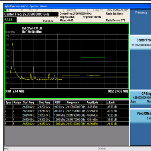
Band38-10MHz-QPSK-38200-1RB#0-PASS
