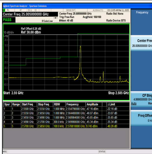
Band38-15MHz-QPSK-37825-75RB#0-PASS
