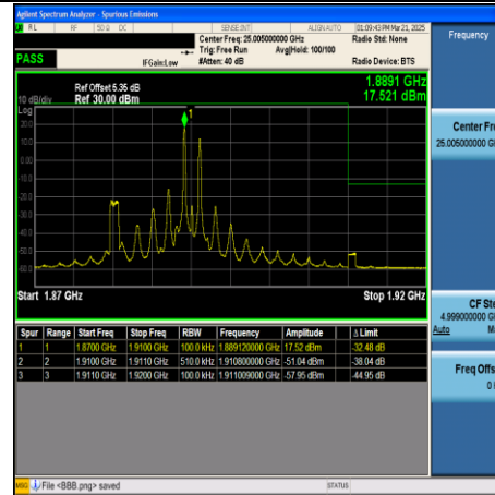
CA_2C-20MHz+20MHz-QPSK-18902+19100- 100RB#0+100RB#0-PASS
