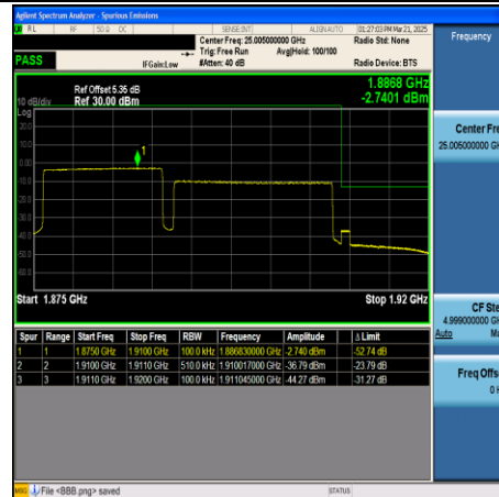
CA_2C-15MHz+20MHz-QPSK-18929+19100- 75RB#0+100RB#0-PASS
