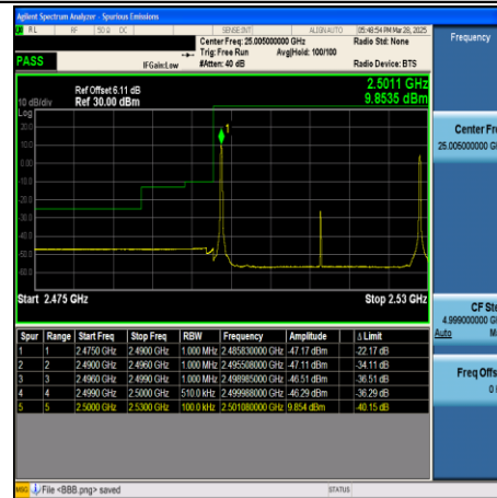
CA_7C-10MHz+20MHz-QPSK-21206+21350- 1RB#49+1RB#0-PASS
