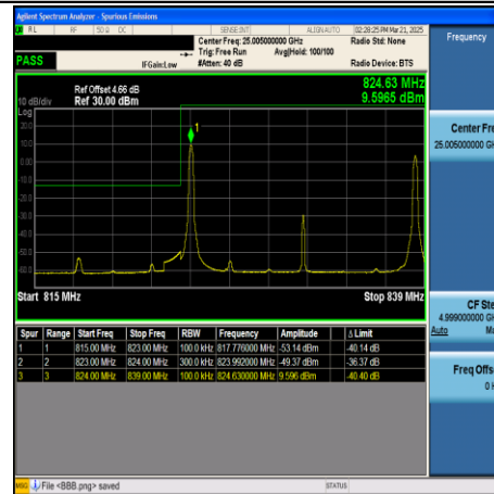
CA_5B-5MHz+10MHz-QPSK-20528+20600- 1RB#24+1RB#0-PASS
