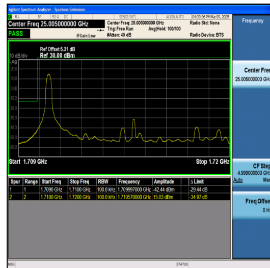
Band66-10MHz-QPSK-132022-50RB#0-PASS
