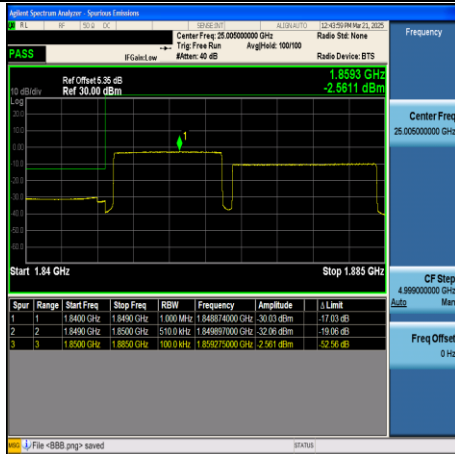
CA_2C-15MHz+20MHz-QPSK-18929+19100- 1RB#0+1RB#99-PASS
