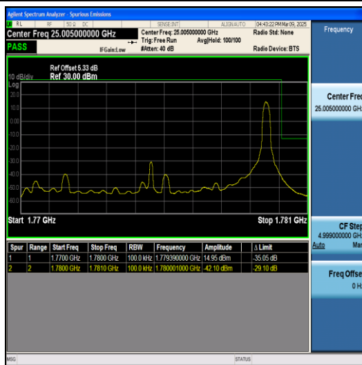
Band66-15MHz-QPSK-132047-1RB#0-PASS
