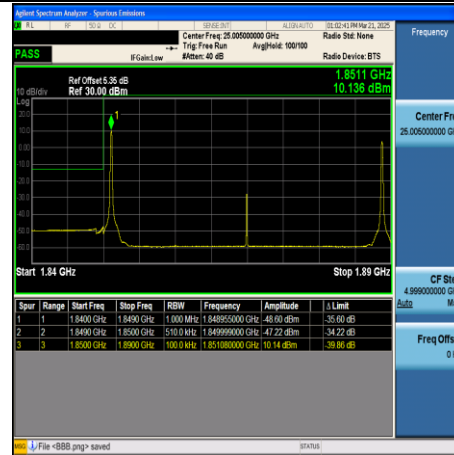
CA_2C-20MHz+20MHz-QPSK-18902+19100- 1RB#99+1RB#0-PASS
