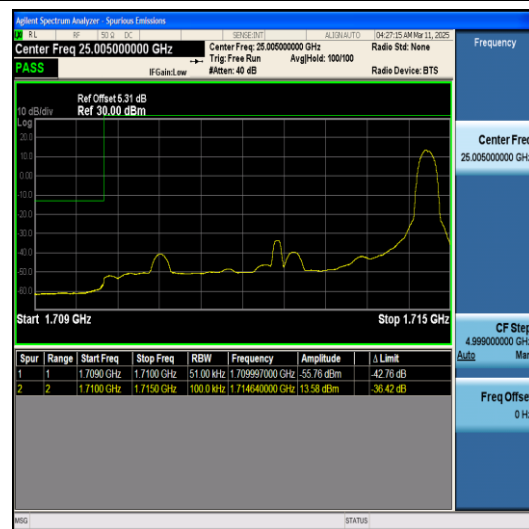
Band66-5MHz-QPSK-132647-1RB#0-PASS
