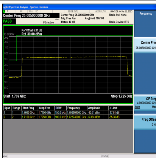
Band66-15MHz-QPSK-132047-75RB#0-PASS
