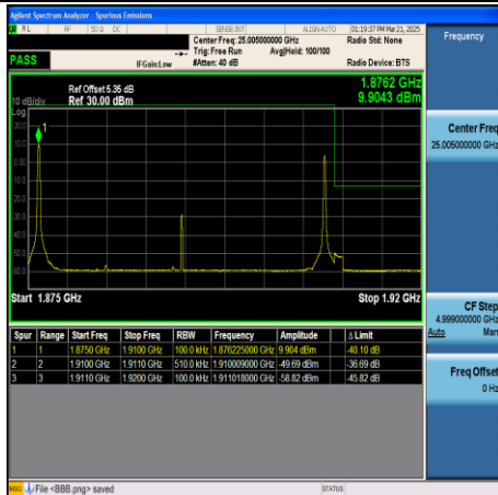
CA_2C-15MHz+20MHz-QPSK-18929+19100- 1RB#0+1RB#99-PASS
