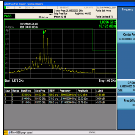
CA_2C-15MHz+20MHz-QPSK-18929+19100- 75RB#0+100RB#0-PASS
