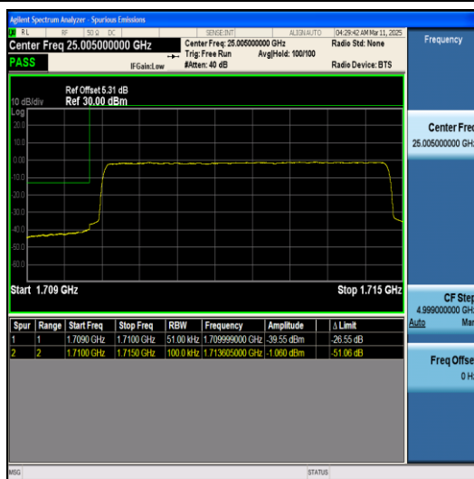
Band66-5MHz-QPSK-131997-25RB#0-PASS
