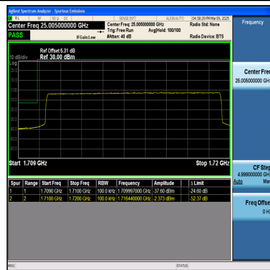
Band66-10MHz-QPSK-132022-50RB#0-PASS
