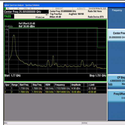
Band66-10MHz-QPSK-132622-1RB#0-PASS
