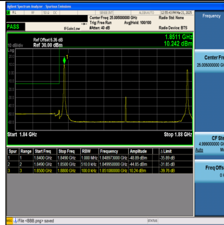
CA_2C-10MHz+20MHz-QPSK-18956+19100- 1RB#49+1RB#0-PASS
