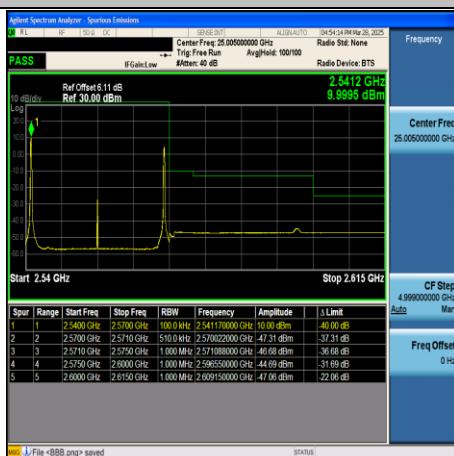
CA_7C-10MHz+20MHz-QPSK-21206+21350- 1RB#0+1RB#99-PASS
