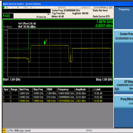
CA_2C-20MHz+20MHz-QPSK-18902+19100- 1RB#0+1RB#99-PASS
