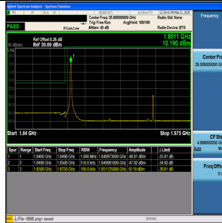
CA_2C-15MHz+20MHz-QPSK-18929+19100- 1RB#74+1RB#0-PASS
