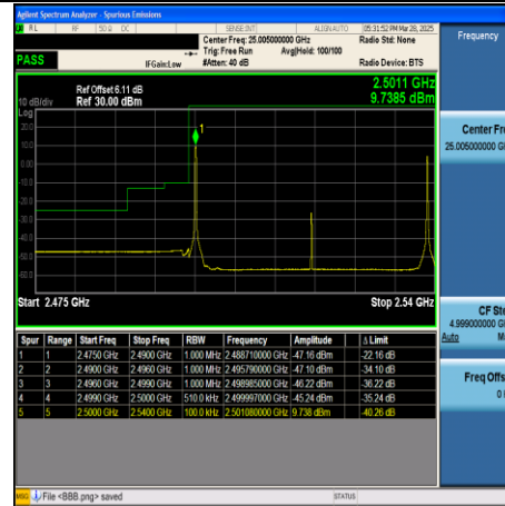
CA_7C-20MHz+20MHz-QPSK-21152+21350- 1RB#99+1RB#0-PASS
