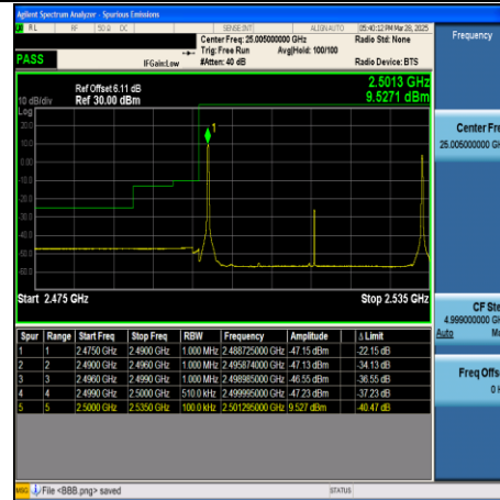
CA_7C-15MHz+20MHz-QPSK-21179+21350- 1RB#74+1RB#0-PASS
