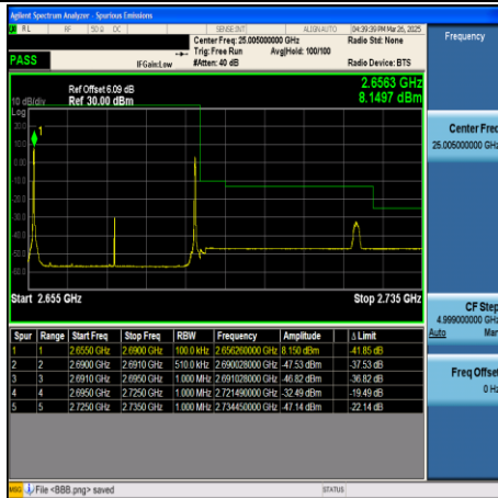
CA_41C-15MHz+20MHz-QPSK-41319+41490- 1RB#0+1RB#99-PASS
