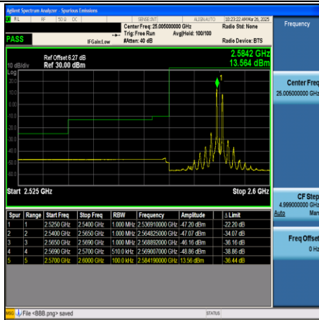
CA_38C-15MHz+15MHz-QPSK-37825+37975- 75RB#0+75RB#0-PASS
