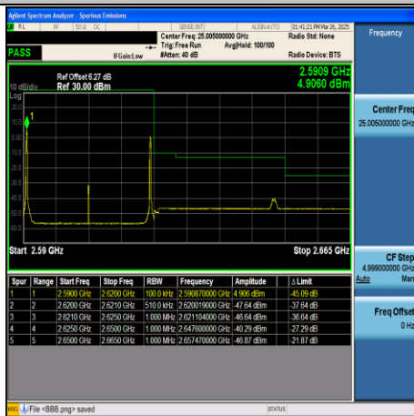
CA_38C-15MHz+15MHz-QPSK-38025+38175- 1RB#0+1RB#74-PASS
