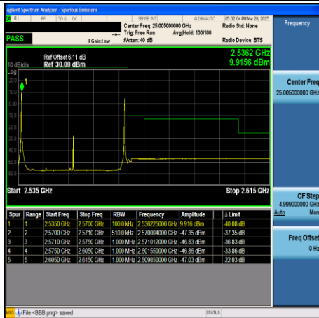
CA_7C-15MHz+20MHz-QPSK-21179+21350- 1RB#0+1RB#99-PASS
