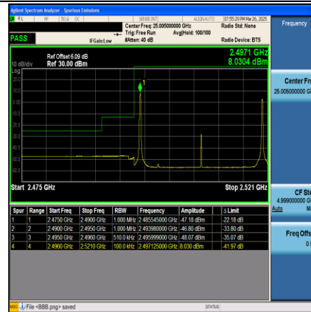
CA_41C-5MHz+20MHz-QPSK-41373+41490- 1RB#24+1RB#0-PASS
