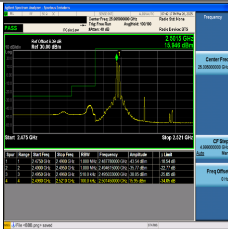
CA_41C-5MHz+20MHz-QPSK-39683+39800- 25RB#0+100RB#0-PASS
