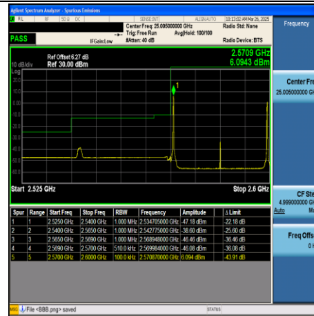
CA_38C-15MHz+15MHz-QPSK-38025+38175- 1RB#74+1RB#0-PASS
