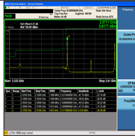
CA_38C-20MHz+20MHz-QPSK-37952+38150- 1RB#99+1RB#0-PASS
