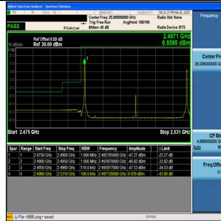
CA_41C-15MHz+20MHz-QPSK-41319+41490- 1RB#74+1RB#0-PASS
