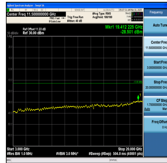
Band66-10MHz-QPSK-132622-1RB#0-3000~2000 0-PASS
