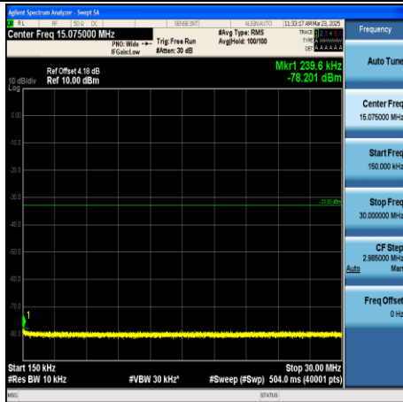
CA_2C-10MHz+20MHz-QPSK-18655+18799- 1RB#49+1RB#0-0.15~30-PASS
