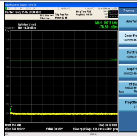
CA_5B-5MHz+10MHz-QPSK-20528+20600- 1RB#24+1RB#0-0.15~30-PASS
