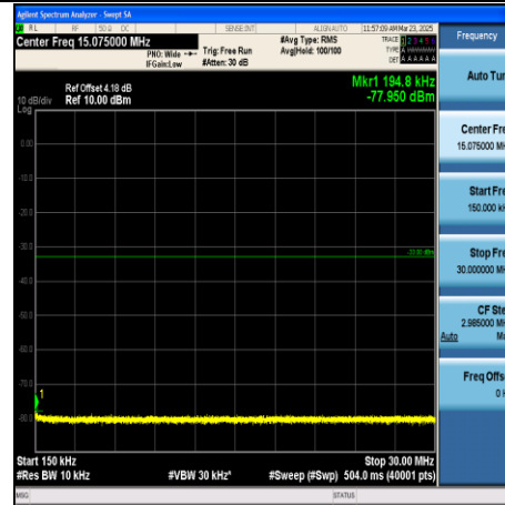
CA_2C-15MHz+20MHz-QPSK-18678+18849- 1RB#74+1RB#0-1000~3000-PASS
