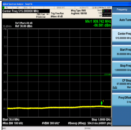
CA_2C-20MHz+20MHz-QPSK-18801+18999- 1RB#99+1RB#0-30~1000-PASS
