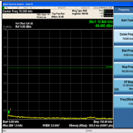
CA_2C-15MHz+20MHz-QPSK-18929+19100- 1RB#74+1RB#0-0.009~0.15-PASS
