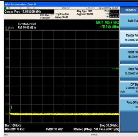
CA_2C-15MHz+20MHz-QPSK-18929+19100- 1RB#74+1RB#0-0.15~30-PASS
