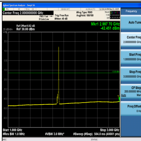
CA_2C-20MHz+20MHz-QPSK-18902+19100- 1RB#99+1RB#0-1000~3000-PASS
