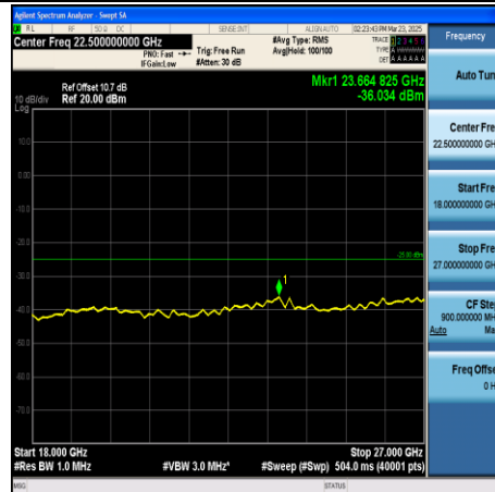
CA_7C-10MHz+20MHz-QPSK-21206+21350- 1RB#49+1RB#0-18000~27000-PASS
