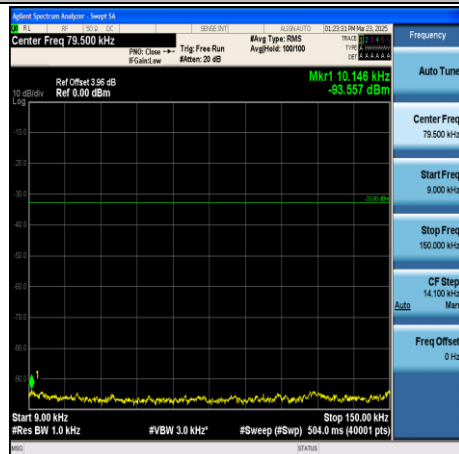
CA_5B-5MHz+10MHz-QPSK-20528+20600- 1RB#24+1RB#0-0.009~0.15-PASS
