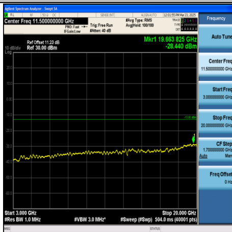
CA_2C-15MHz+20MHz-QPSK-18678+18849- 1RB#74+1RB#0-3000~20000-PASS
