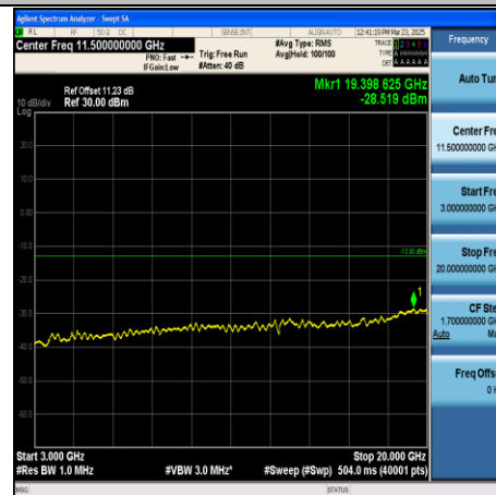
CA_2C-20MHz+20MHz-QPSK-18902+19100- 1RB#99+1RB#0-3000~20000-PASS
