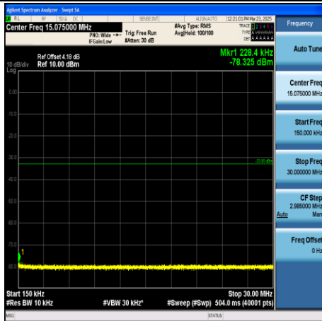
CA_2C-20MHz+20MHz-QPSK-18700+18898- 1RB#99+1RB#0-0.15~30-PASS
