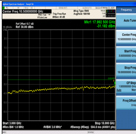
CA_7C-10MHz+20MHz-QPSK-21206+21350- 1RB#49+1RB#0-3000~18000-PASS
