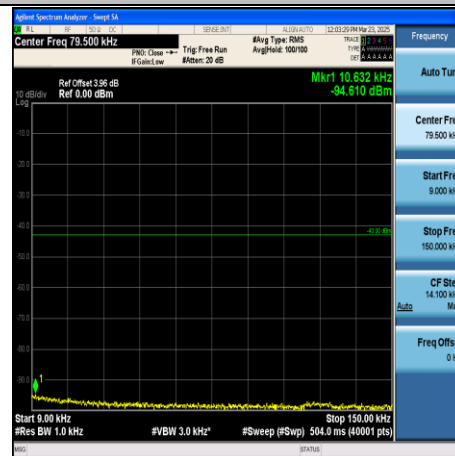
CA_2C-15MHz+20MHz-QPSK-18803+18974- 1RB#74+1RB#0-0.009~0.15-PASS
