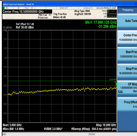
CA_7C-10MHz+20MHz-QPSK-21006+21150- 1RB#49+1RB#0-3000~18000-PASS
