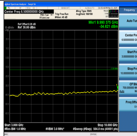
CA_5B-10MHz+10MHz-QPSK-20501+20600- 1RB#49+1RB#0-3000~10000-PASS
