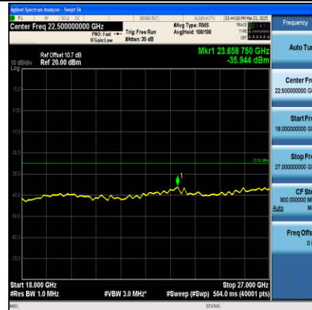
CA_38C-15MHz+15MHz-QPSK-37925+38075- 1RB#74+1RB#0-18000~27000-PASS
