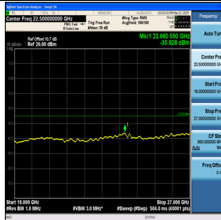
CA_7C-20MHz+20MHz-QPSK-20850+21048- 1RB#99+1RB#0-18000~27000-PASS
