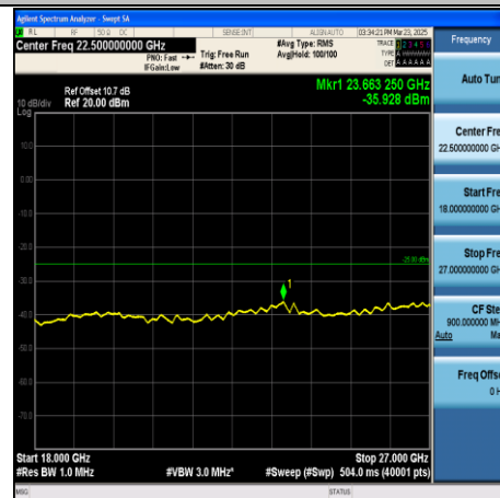
CA_38C-15MHz+15MHz-QPSK-37825+37975- 1RB#74+1RB#0-18000~27000-PASS
