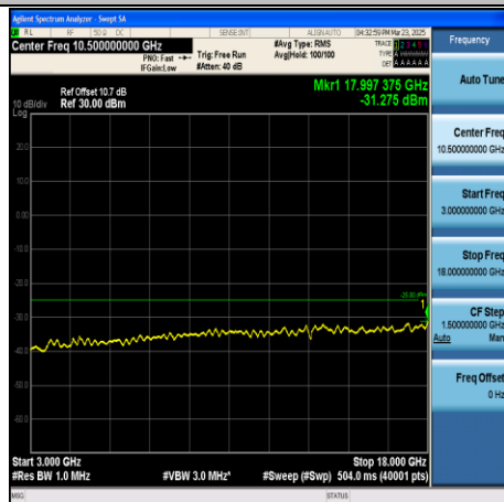
CA_41C-5MHz+20MHz-QPSK-39683+39800- 1RB#24+1RB#0-3000~18000-PASS
