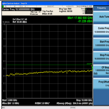
CA_38C-20MHz+20MHz-QPSK-37901+38099- 1RB#99+1RB#0-3000~18000-PASS
