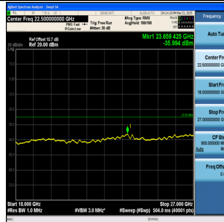
CA_38C-20MHz+20MHz-QPSK-37901+38099- 1RB#99+1RB#0-18000~27000-PASS
