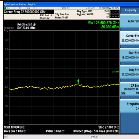
CA_7C-20MHz+20MHz-QPSK-21152+21350- 1RB#99+1RB#0-18000~27000-PASS
