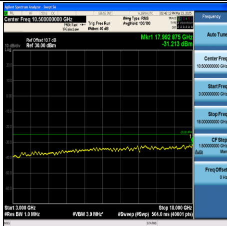
CA_38C-15MHz+15MHz-QPSK-37925+38075- 1RB#74+1RB#0-3000~18000-PASS
