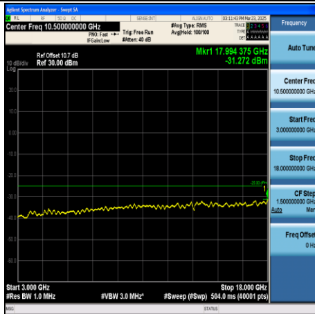
CA_7C-20MHz+20MHz-QPSK-21001+21199- 1RB#99+1RB#0-3000~18000-PASS
