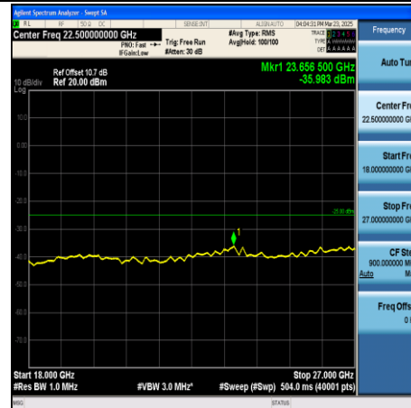
CA_38C-20MHz+20MHz-QPSK-37850+38048- 1RB#99+1RB#0-18000~27000-PASS
