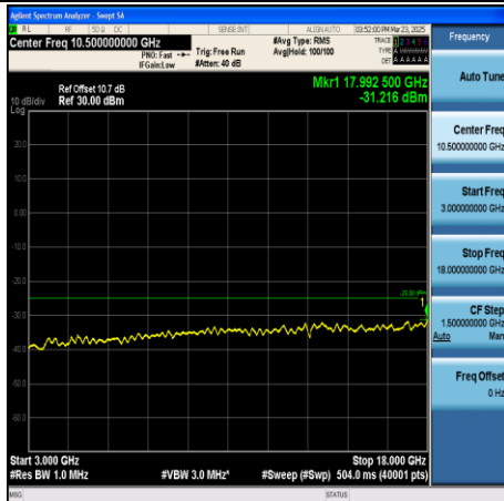
CA_38C-15MHz+15MHz-QPSK-38025+38175- 1RB#74+1RB#0-3000~18000-PASS
