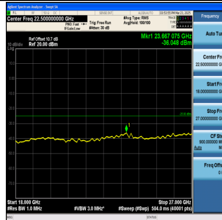
CA_38C-15MHz+15MHz-QPSK-38025+38175- 1RB#74+1RB#0-18000~27000-PASS
