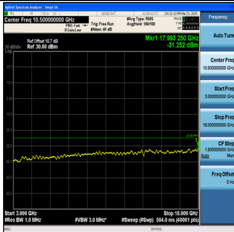
CA_38C-20MHz+20MHz-QPSK-37952+38150- 1RB#99+1RB#0-3000~18000-PASS
