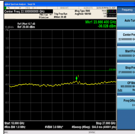
CA_7C-15MHz+20MHz-QPSK-21179+21350- 1RB#74+1RB#0-18000~27000-PASS
