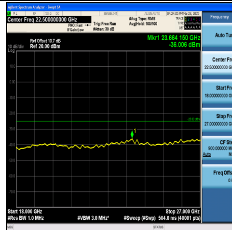
CA_38C-20MHz+20MHz-QPSK-37952+38150- 1RB#99+1RB#0-18000~27000-PASS
