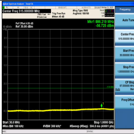
CA_7C-20MHz+20MHz-QPSK-21152+21350- 1RB#99+1RB#0-3000~18000-PASS
