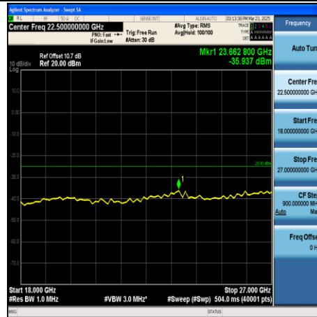
CA_7C-20MHz+20MHz-QPSK-21001+21199- 1RB#99+1RB#0-18000~27000-PASS
