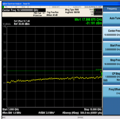
CA_7C-20MHz+20MHz-QPSK-20850+21048- 1RB#99+1RB#0-3000~18000-PASS
