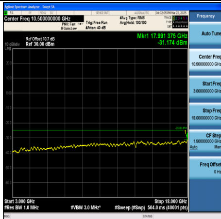
CA_38C-20MHz+20MHz-QPSK-37850+38048- 1RB#99+1RB#0-3000~18000-PASS
