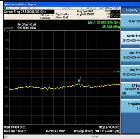
CA_7C-15MHz+20MHz-QPSK-21003+21174- 1RB#74+1RB#0-18000~27000-PASS
