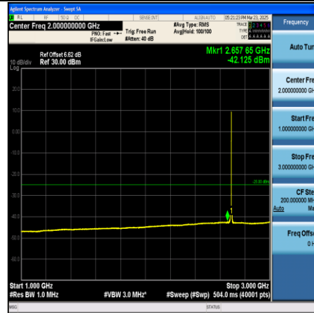
CA_41C-10MHz+20MHz-QPSK-41319+41490- 1RB#49+1RB#0-18000~27000-PASS
