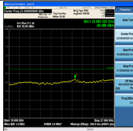
CA_41C-15MHz+20MHz-QPSK-41319+41490- 1RB#74+1RB#0-18000~27000-PASS
