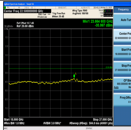
CA_41C-15MHz+20MHz-QPSK-40523+40694- 1RB#74+1RB#0-18000~27000-PASS
