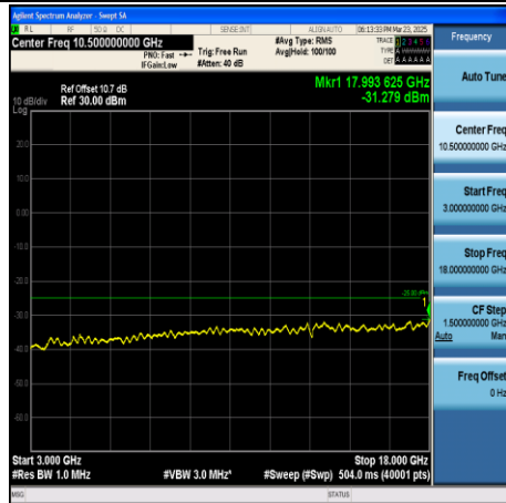
CA_41C-20MHz+20MHz-QPSK-40521+40719- 1RB#99+1RB#0-3000~18000-PASS
