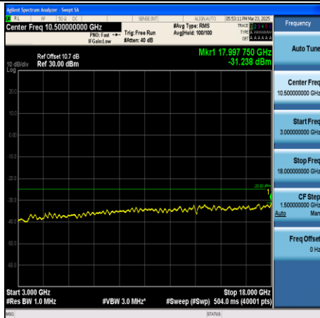
CA_41C-15MHz+20MHz-QPSK-41319+41490- 1RB#74+1RB#0-3000~18000-PASS
