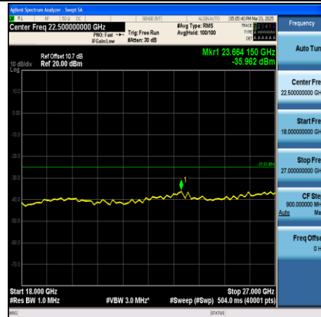
CA_41C-10MHz+20MHz-QPSK-39705+39849- 1RB#49+1RB#0-18000~27000-PASS
