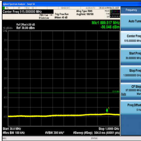
CA_41C-15MHz+20MHz-QPSK-39728+39899- 1RB#74+1RB#0-3000~18000-PASS
