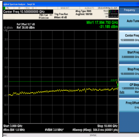
CA_41C-10MHz+20MHz-QPSK-39705+39849- 1RB#49+1RB#0-3000~18000-PASS
