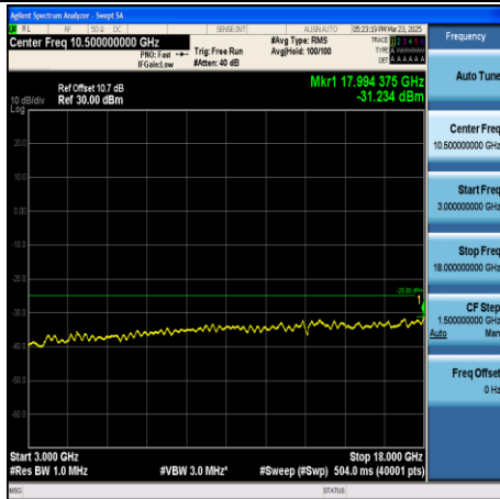
CA_41C-10MHz+20MHz-QPSK-41319+41490- 1RB#49+1RB#0-3000~18000-PASS
