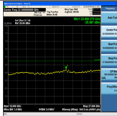
CA_41C-5MHz+20MHz-QPSK-41373+41490- 1RB#24+1RB#0-18000~27000-PASS
