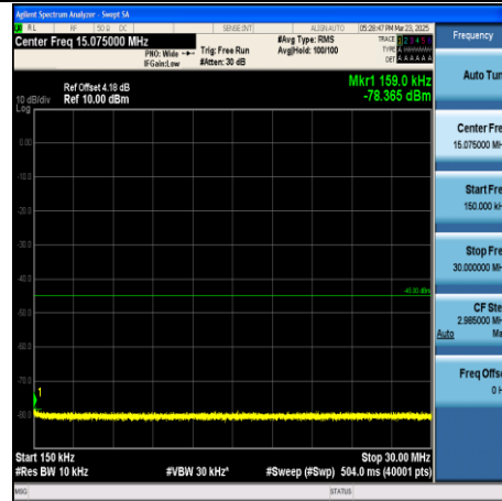
CA_41C-15MHz+20MHz-QPSK-39728+39899- 1RB#74+1RB#0-1000~3000-PASS
