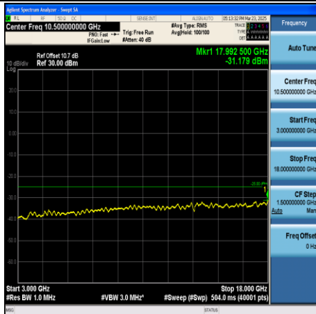
CA_41C-10MHz+20MHz-QPSK-40526+40670- 1RB#49+1RB#0-3000~18000-PASS
