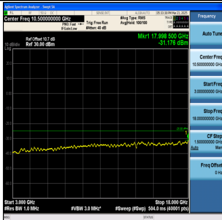
CA_41C-15MHz+20MHz-QPSK-39728+39899- 1RB#74+1RB#0-3000~18000-PASS
