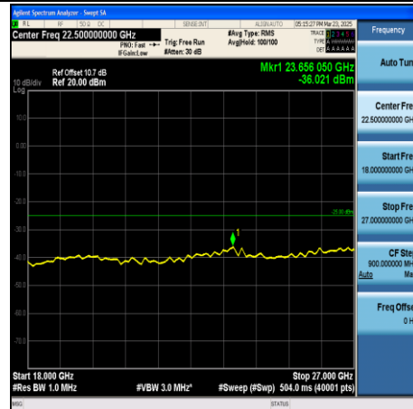
CA_41C-10MHz+20MHz-QPSK-40526+40670- 1RB#49+1RB#0-18000~27000-PASS
