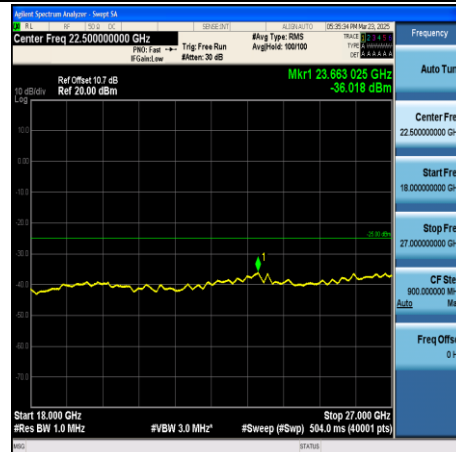
CA_41C-15MHz+20MHz-QPSK-39728+39899- 1RB#74+1RB#0-18000~27000-PASS
