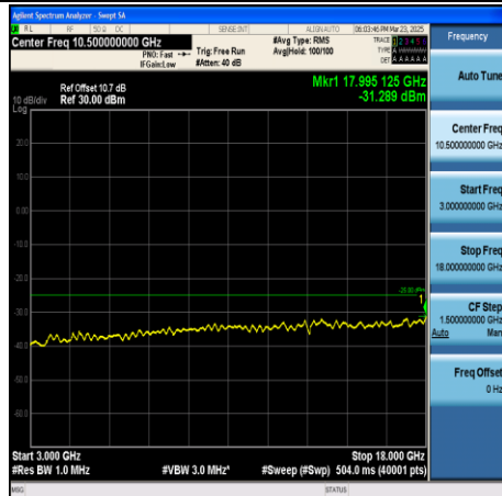
CA_41C-20MHz+20MHz-QPSK-39750+39948- 1RB#99+1RB#0-3000~18000-PASS
