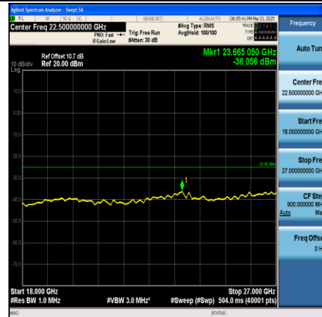
CA_41C-20MHz+20MHz-QPSK-39750+39948- 1RB#99+1RB#0-18000~27000-PASS
