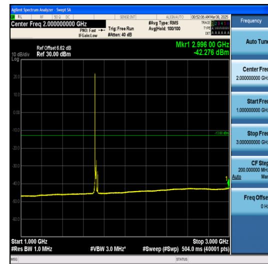
Band4-15MHz-QPSK-20025-1RB#0-1000~3000-P
