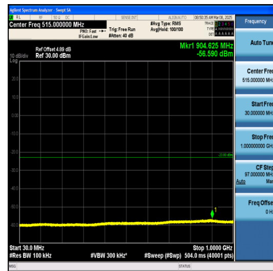
Band4-15MHz-QPSK-20025-1RB#0-30~1000-PA
