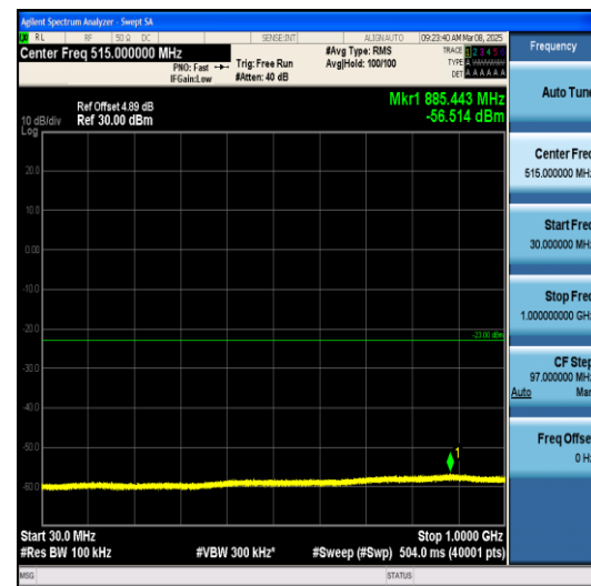
Band4-20MHz-QPSK-20175-1RB#0-30~1000-PA
