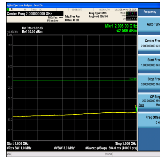
Band5-3MHz-QPSK-20525-1RB#0-1000~3000-PA SS
