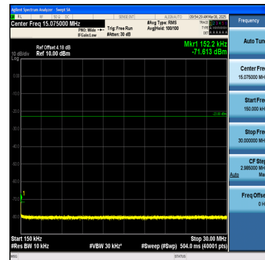
Band5-1.4MHz-QPSK-20643-1RB#0-0.15~30-PAS
