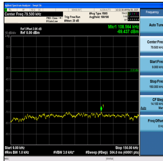
Band5-5MHz-QPSK-20525-1RB#0-0.009~0.15-P ASS
