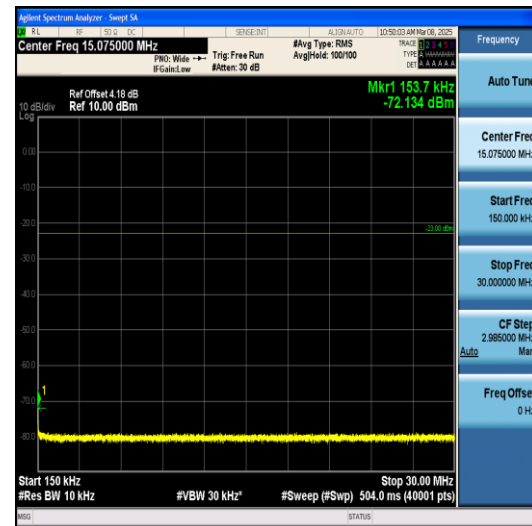
Band5-10MHz-QPSK-20450-1RB#0-0.15~30-PAS S
