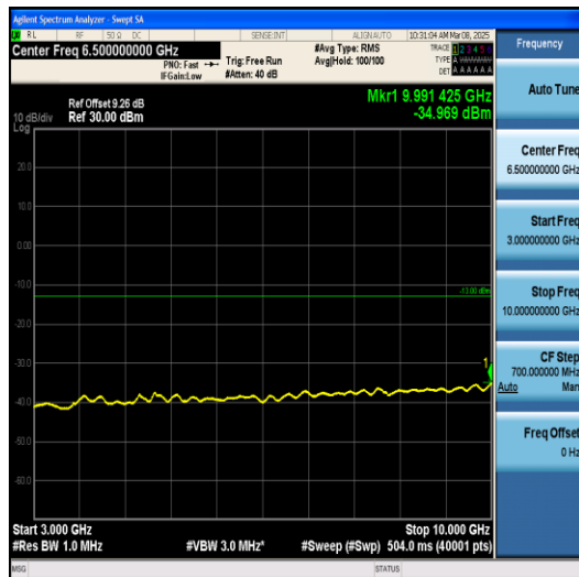
Band5-5MHz-QPSK-20425-1RB#0-3000~10000-P ASS
