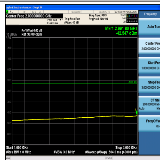
Band5-5MHz-QPSK-20625-1RB#0-1000~3000-PA SS
