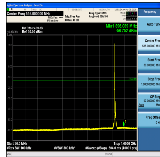
Band5-10MHz-QPSK-20450-1RB#0-30~1000-PA SS
