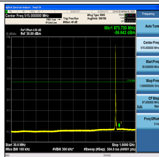
Band5-5MHz-QPSK-20625-1RB#0-30~1000-PAS S
