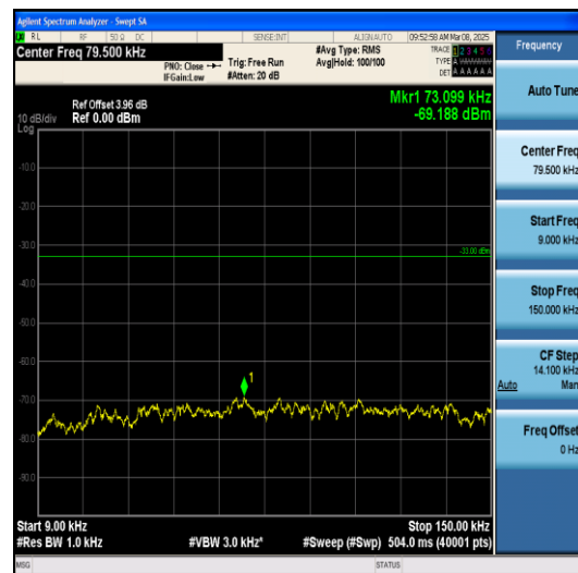
Band5-1.4MHz-QPSK-20643-1RB#0-0.009~0.15-PASS
