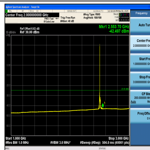
Band7-15MHz-QPSK-20825-1RB#0-1000~3000-P
