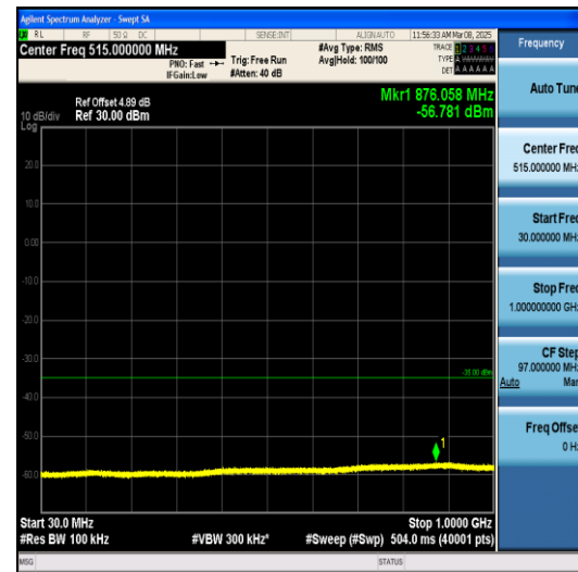
Band7-10MHz-QPSK-21100-1RB#0-30~1000-PAS
