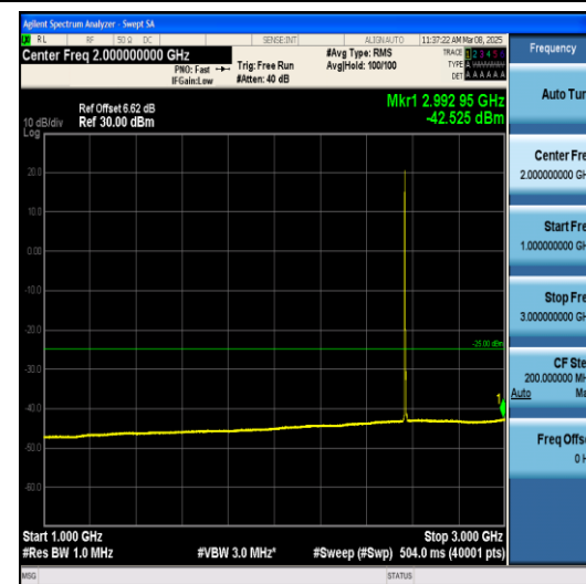
Band7-5MHz-QPSK-21425-1RB#0-1000~3000-PA SS
