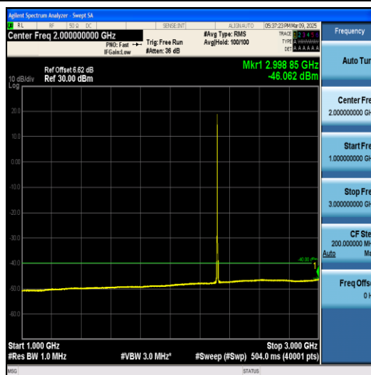
Band40(2305-2320)-10MHz-QPSK-38750-1RB#0 -0.009~0.15-PASS
