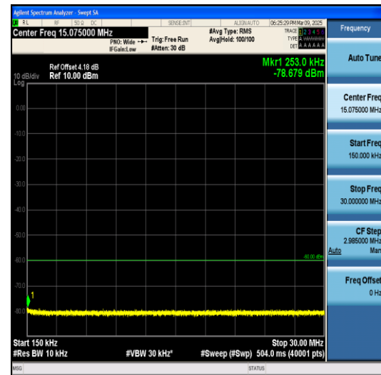
Band40(2345-2360)-5MHz-QPSK-39175-1RB#0- 0.15~30-PASS
