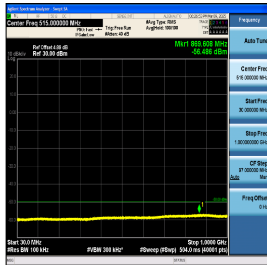
Band40(2345-2360)-5MHz-QPSK-39175-1RB#0-30 ~1000-PASS
