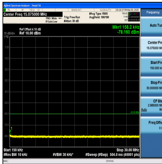
Band40(2305-2320)-5MHz-QPSK-38775-1RB #0-0.15~30-PASS
