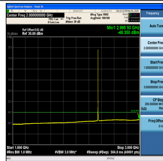
Band40(2345-2360)-5MHz-QPSK-39125-1RB#0-1 000~3000-PASS
