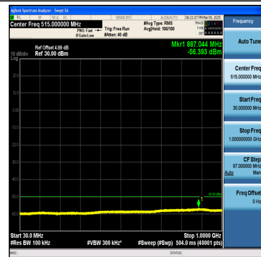
Band40(2345-2360)-5MHz-QPSK-39125-1RB#0-3 0~1000-PASS
