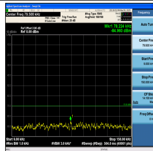
Band40(2305-2320)-10MHz-QPSK-38750-1RB#0 -0.009~0.15-PASS
