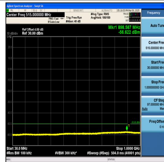
Band40(2305-2320)-5MHz-QPSK-38725-1RB#0-3 0~1000-PASS
