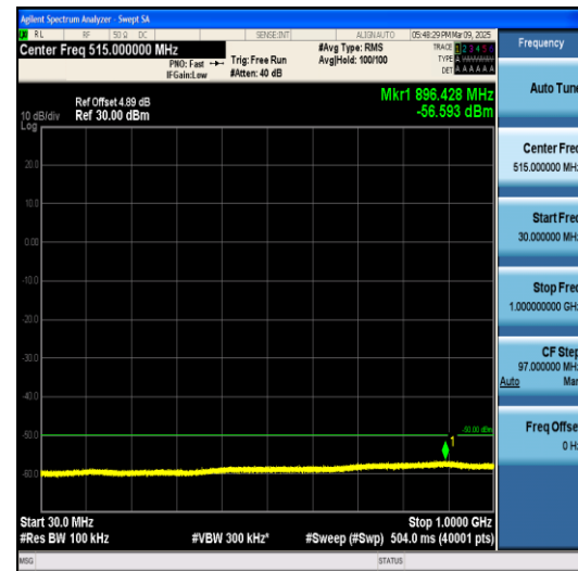
Band40(2305-2320)-10MHz-QPSK-38775-1RB#0- 30~1000-PASS
