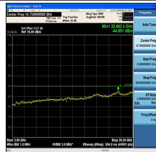
Band40(2305-2320)-5MHz-QPSK-38825-1RB#0-3 000~26500-PASS
