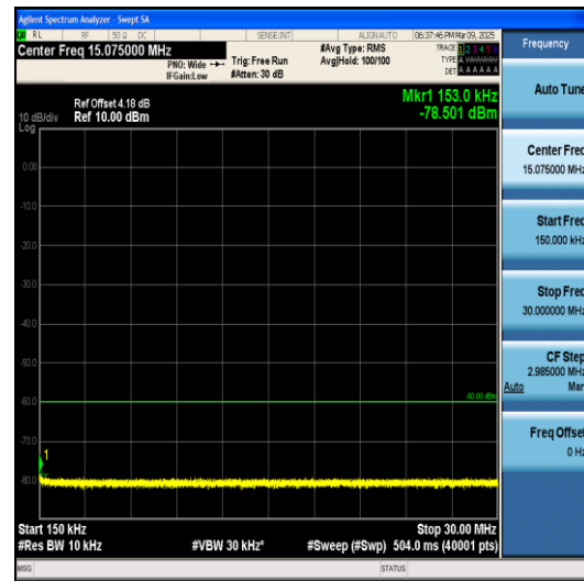
Band40(2345-2360)-10MHz-QPSK-39150-1RB#0 -1000~3000-PASS
