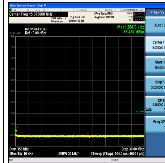
Band40(2305-2320)-5MHz-QPSK-38825-1RB#0-0. 0.15~30-PASS
