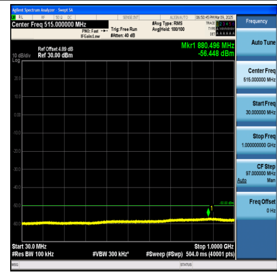
Band40(2345-2360)-10MHz-QPSK-39200-1RB#0- 30~1000-PASS
