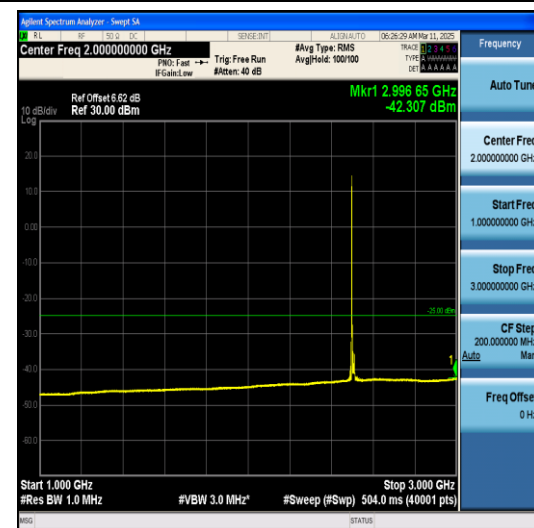
Band41-15MHz-QPSK-39725-1RB#0-1000~3000-
