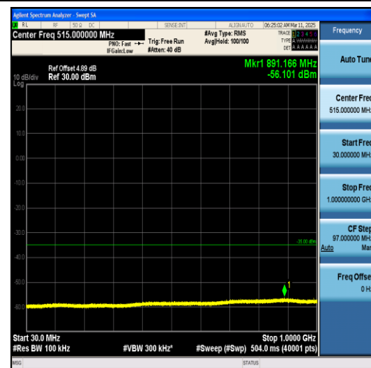
Band41-15MHz-QPSK-39725-1RB#0-30~1000-PA
