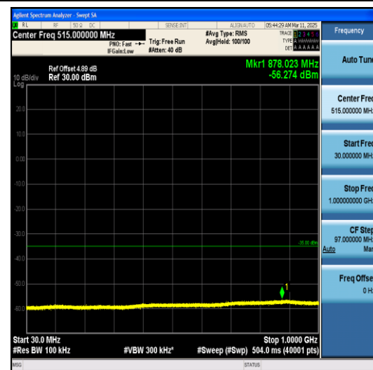
Band41-5MHz-QPSK-41565-1RB#0-30~1000-PA
