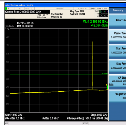
Band41-5MHz-QPSK-41565-1RB#0-1000~3000-P
