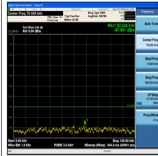
Band40(2345-2360)-10MHz-QPSK-39200-1RB#0- -0.009~0.15-PASS
