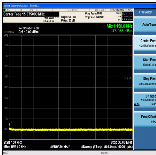
Band66-1.4MHz-QPSK-132322-1RB#0-0.15~30-P ASS
