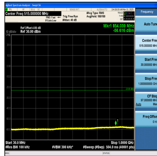
Band66-3MHz-QPSK-132322-1RB#0-30~1000-PA
