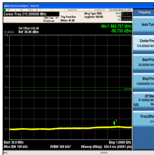
Band66-1.4MHz-QPSK-132322-1RB#0-30~1000- PASS
