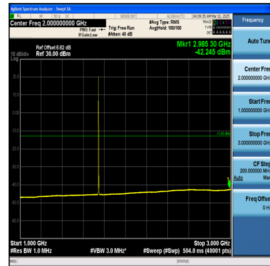
Band66-3MHz-QPSK-132322-1RB#0-1000~3000-
