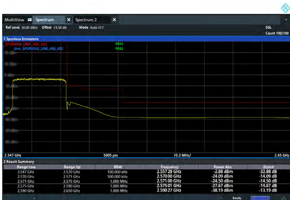
BE_n7_20M_High CH_DL536000_2560MHz_CP_QPSK_Full RB
