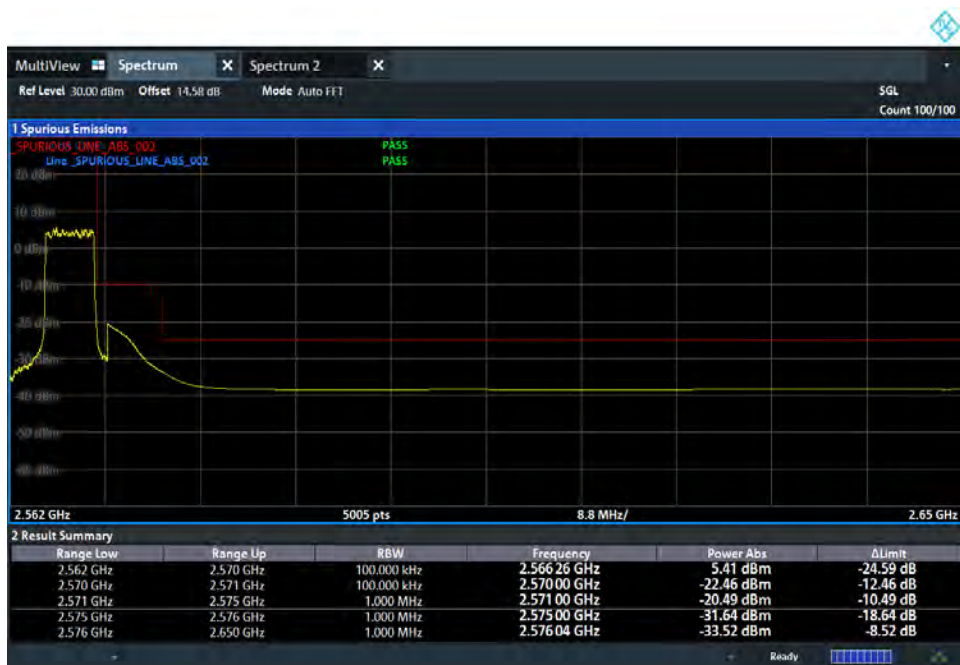
BE_n7_5M_High CH_DL537500_2567.5MHz_DFT_QPSK_Full RB
