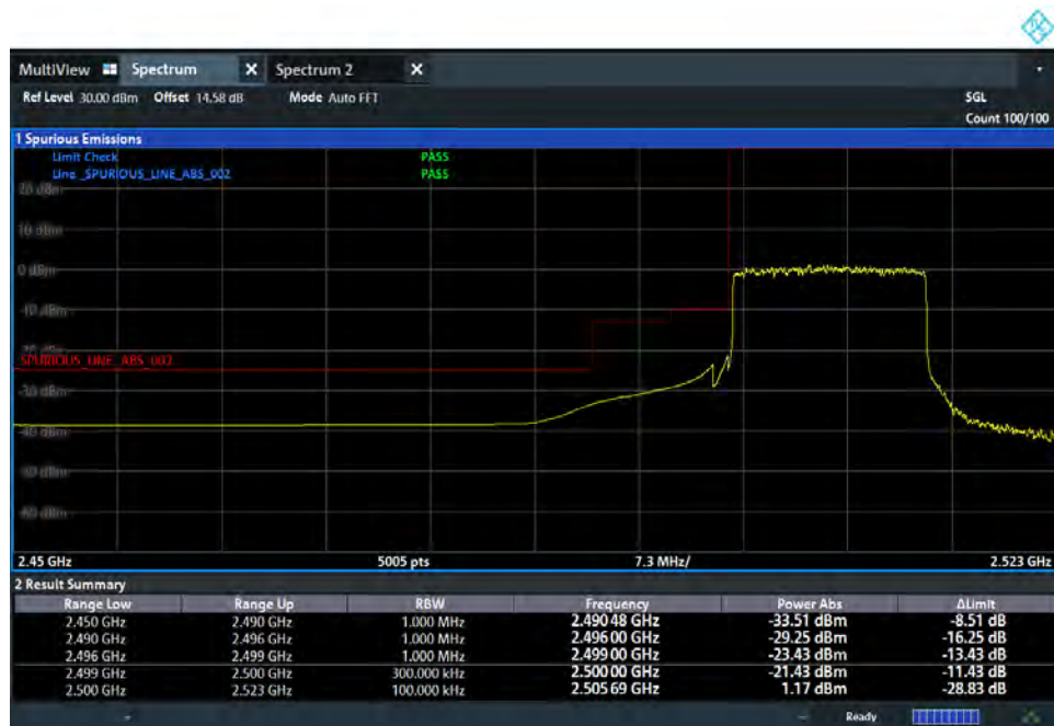
BE_n7_15M_Low CH_DL525500_2507.5MHz_DFT_QPSK_Full RB
