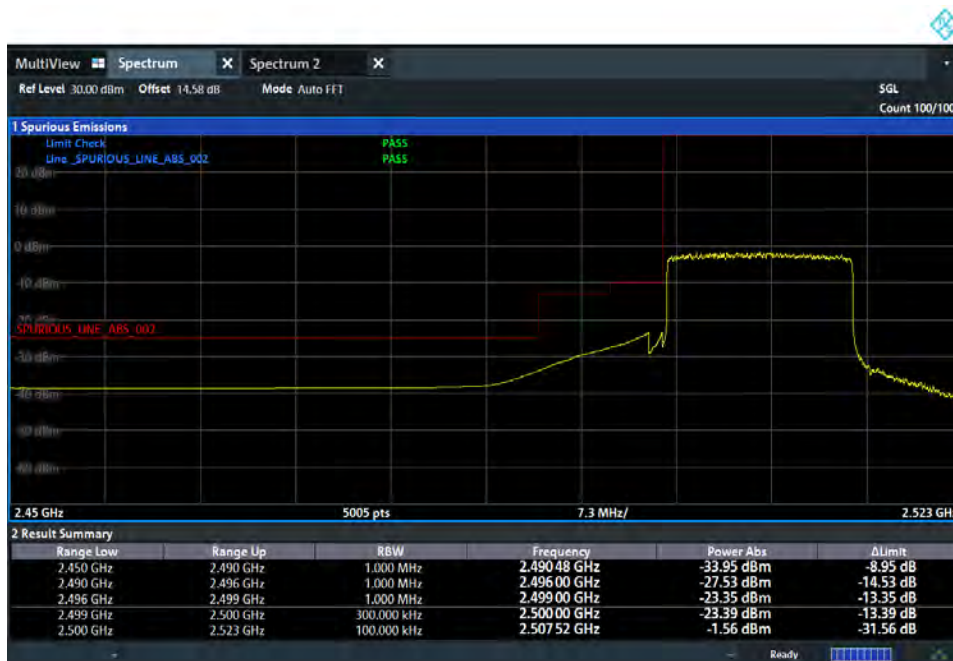
BE_n7_15M_Low CH_DL525500_2507.5MHz_CP_QPSK_Full RB
