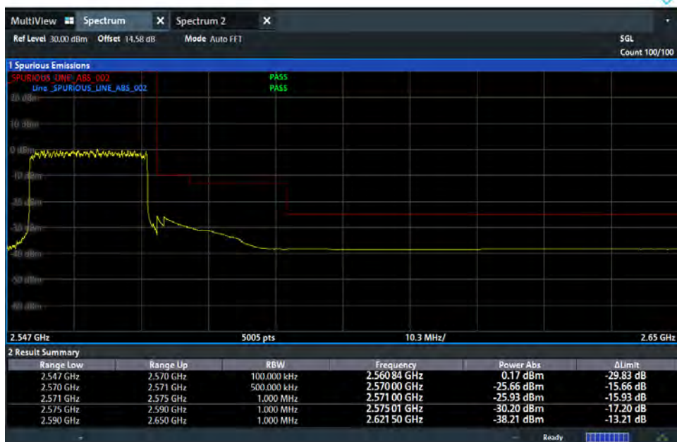
BE_n7_20M_High CH_DL536000_2560MHz_DFT_QPSK_Full RB
