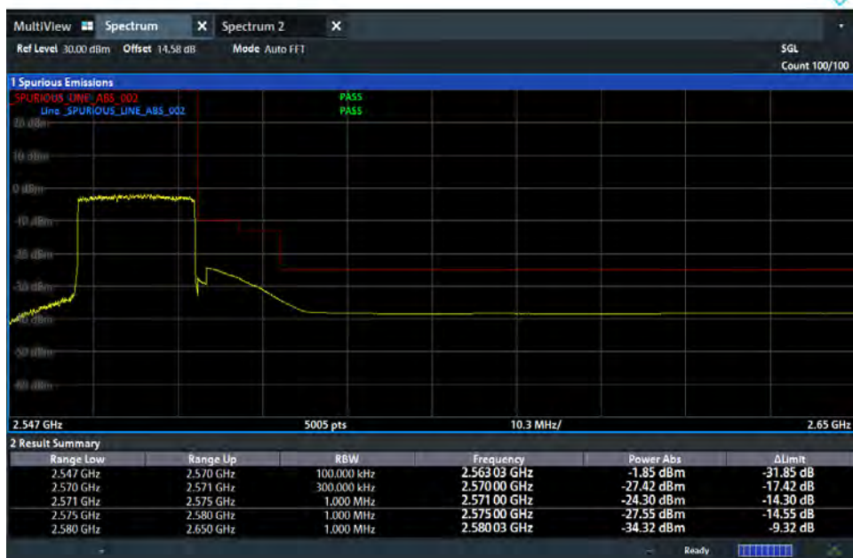
BE_n7_15M_High CH_DL536500_2562.5MHz_CP_QPSK_Full RB
