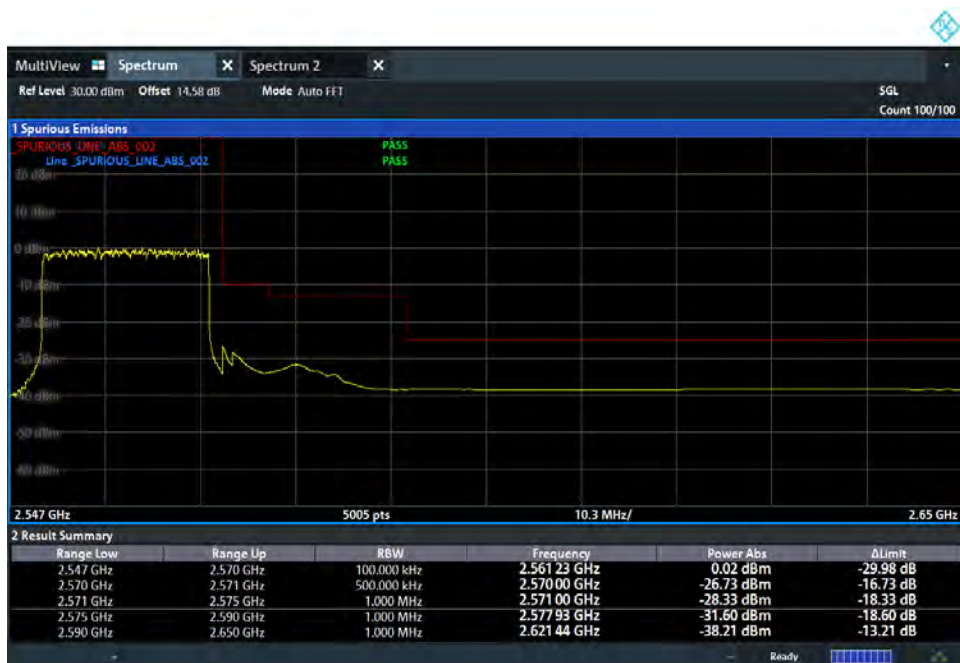
BE_n7_20M_High CH_DL536000_2560MHz_DFT_BPSK_Full RB
