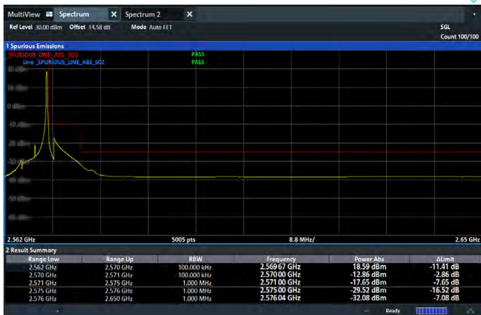
BE_n7_5M_High CH_DL537500_2567.5MHz_DFT_BPSK_Full RB
