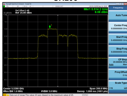
CH106
