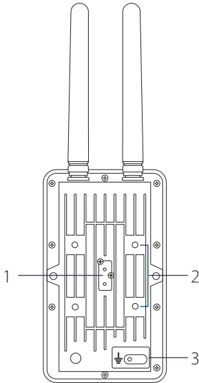
Figure 3: Back Connectors
