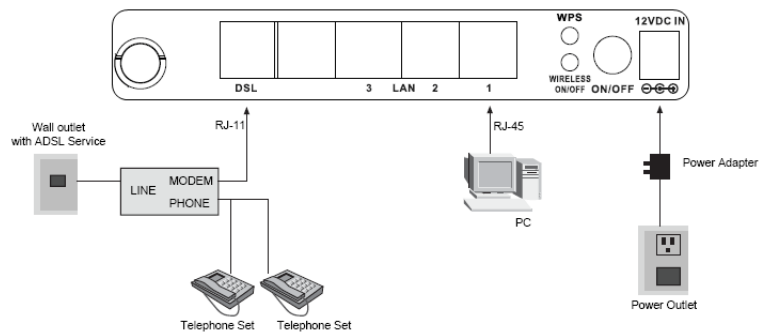
Figure 3 Connection diagram
