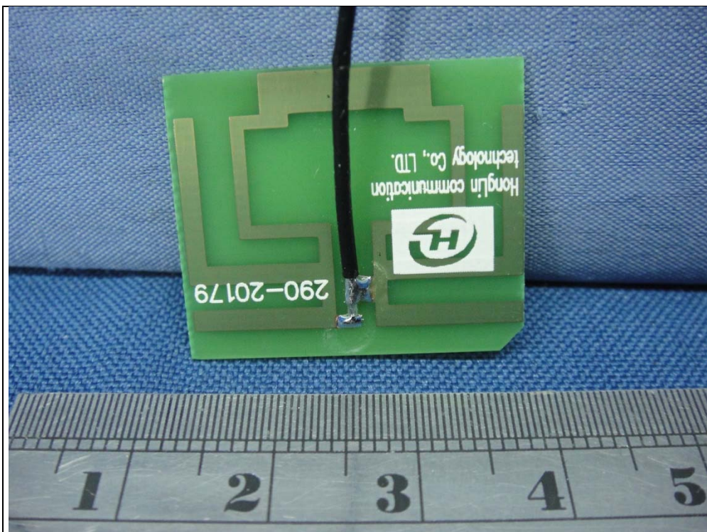
Antenna 1 (Model: 290-20179)
