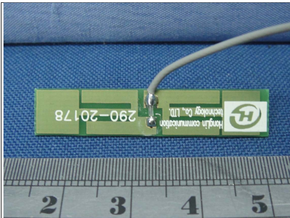
Antenna 2 (Model: 290-20178)
