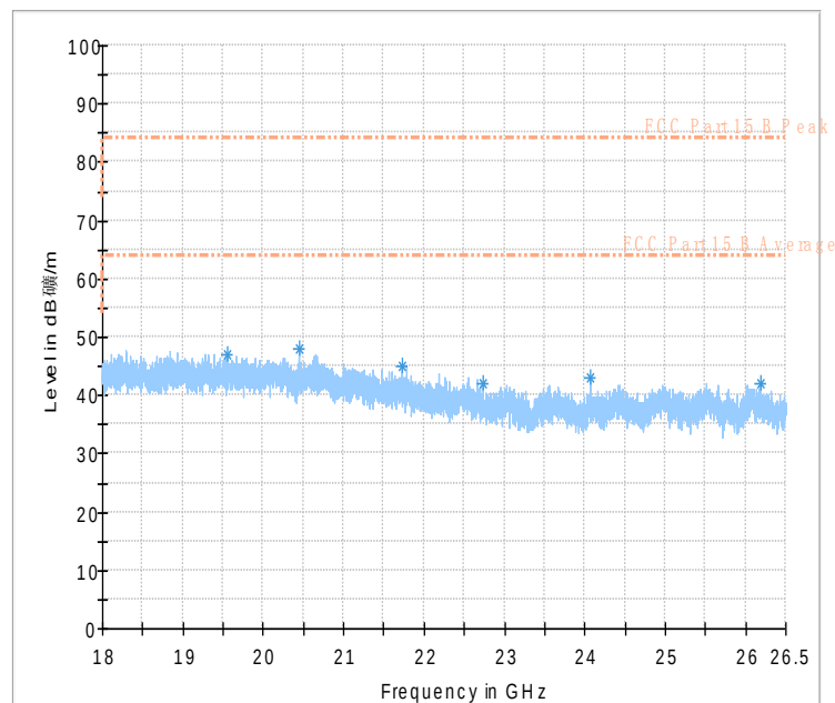
Fig.46 Radiated emission: GFSK, 18 GHz – 26.5 GHz
