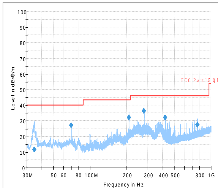
Fig.43 Radiated Spurious Emission (802.11 n-20MHz,Ch1,30MHz~1GHz)
