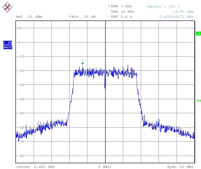
Fig.2 Power Spectral Density (802.1g,Ch11)
