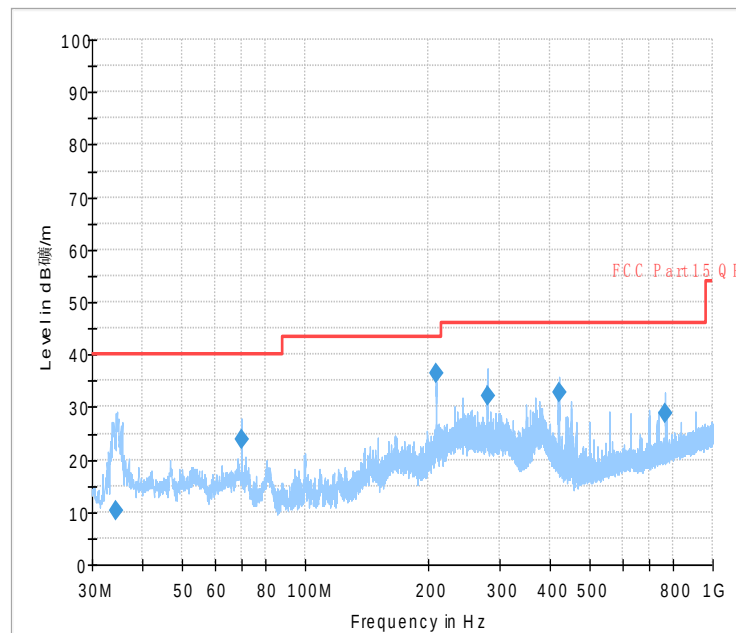
Fig.33 Radiated Spurious Emission (802.11b,Ch1,30MHz~1GHz)
