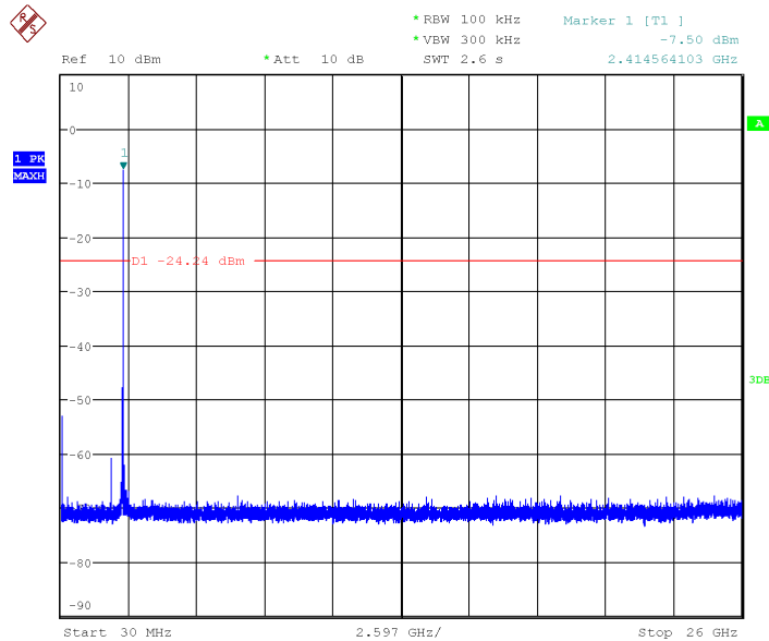
Fig.25 Conducted Spurious Emission (802.11n-20MHz, Ch1)
