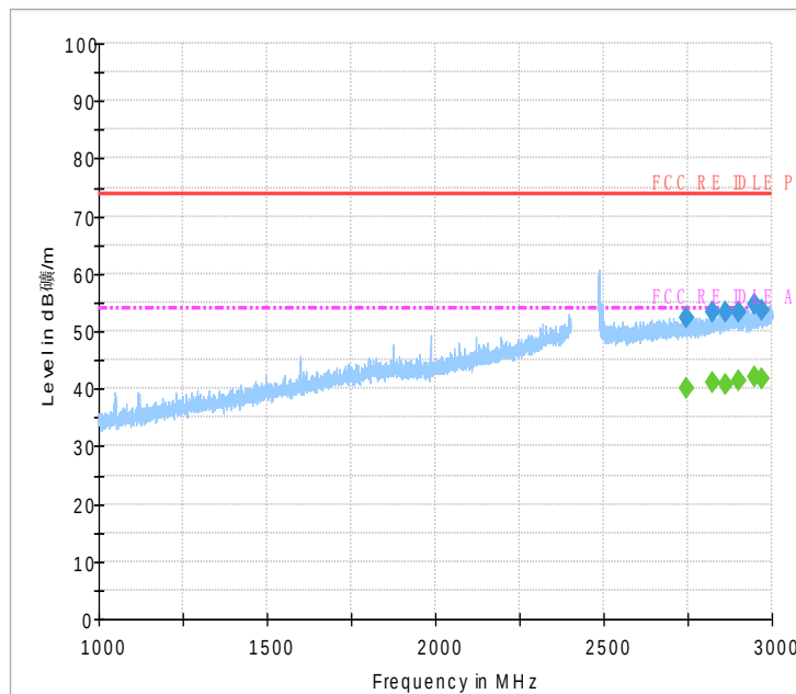
Fig.39 Radiated Spurious Emission (802.11g,Ch11,1GHz~3GHz)
