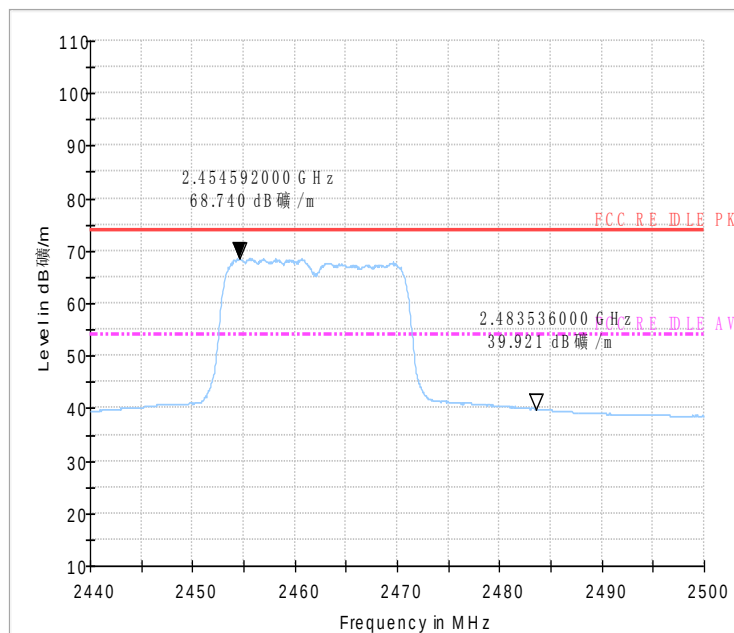
Fig.42 Radiated emission (Power): 802.11n, high channel
