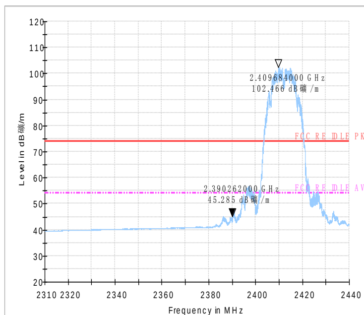
Fig.31 Radiated emission (Power): 802.11b, low channel
