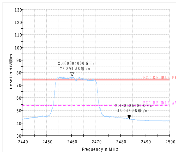
Fig.37 Radiated emission (Power): 802.11g, high channel
