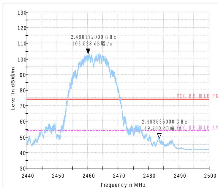
Fig.32 Radiated emission (Power): 802.11b, high channel
