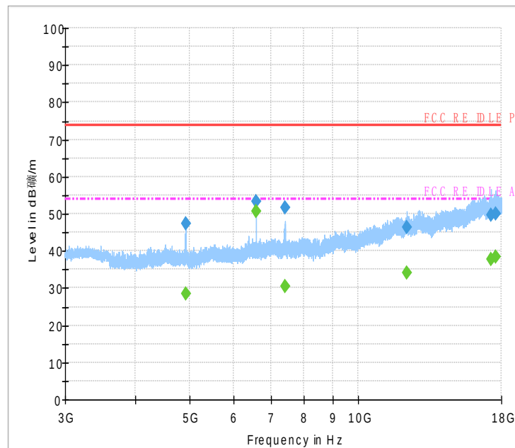
Fig.45 Radiated Spurious Emission (802.11 n-20MHz,Ch1,3GHz~18GHz)
