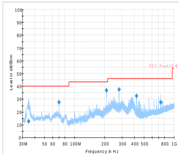
Fig.38 Radiated Spurious Emission (802.11g,Ch11,30MHz~1GHz)
