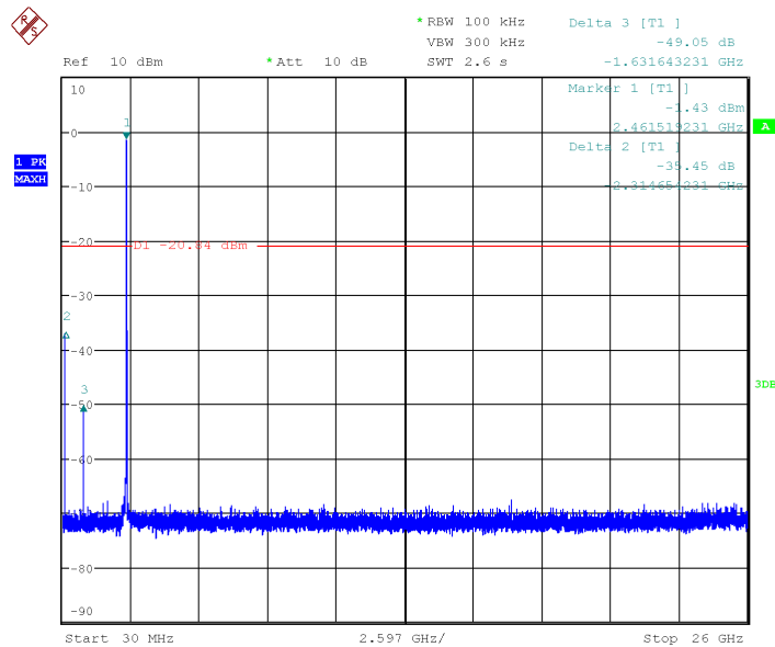
Fig.17 Conducted Spurious Emission (802.11b, Ch11)
