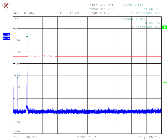
Fig.23 Conducted Spurious Emission (802.11g, Ch11)
