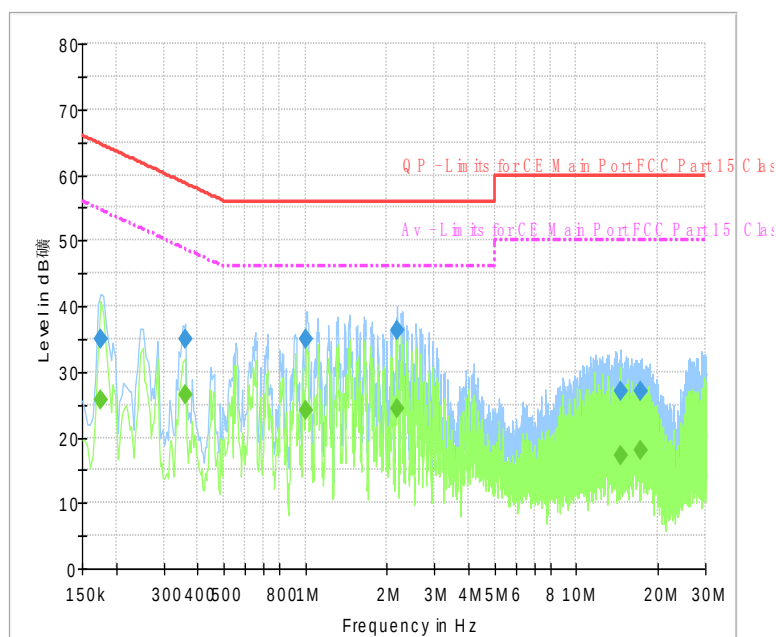
Fig.48 AC AC Powerline Conducted Emission Idle
