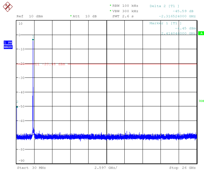
Fig.19 Conducted Spurious Emission (802.11g, Ch1)
