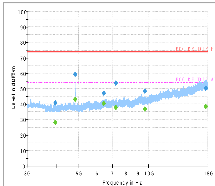
Fig.35 Radiated Spurious Emission (802.11b,Ch1,3GHz~18GHz)
