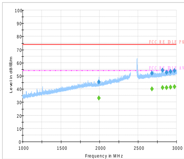
Fig.44 Radiated Spurious Emission (802.11 n-20MHz,Ch1,1GHz~3GHz)
