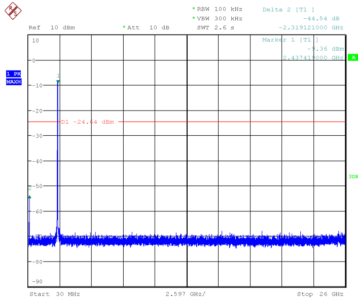
Fig.21 Conducted Spurious Emission (802.11g, Ch6)
