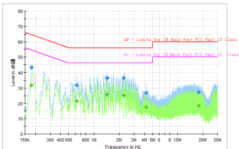
Fig.47 AC Powerline Conducted Emission 802.11n
