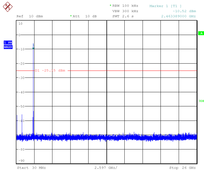
Fig.29 Conducted Spurious Emission (802.11n-20MHz, Ch11)
