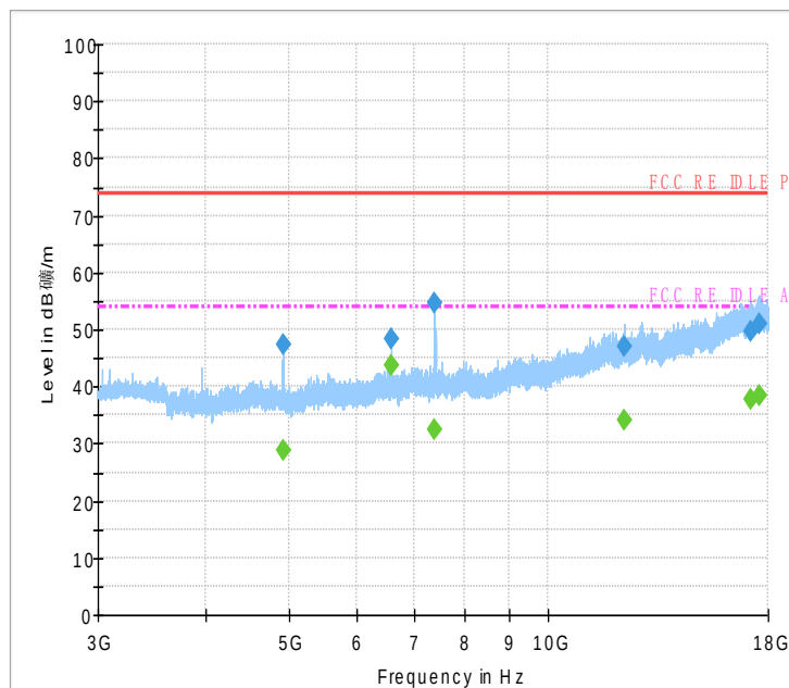
Fig.40 Radiated Spurious Emission (802.11g,Ch11,3GHz~18GHz)
