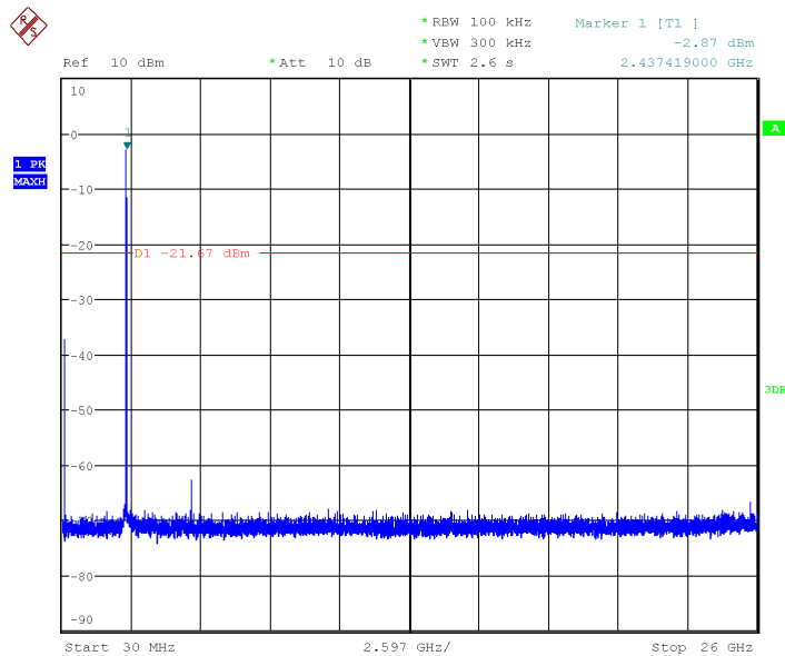
Fig.15 Conducted Spurious Emission (802.11b, Ch6)
