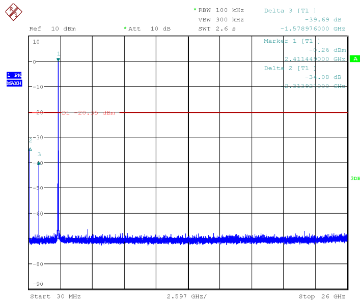
Fig.13 Conducted Spurious Emission (802.11b, Ch1)
