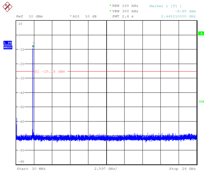
Fig.27 Conducted Spurious Emission (802.11n-20MHz, Ch6)
