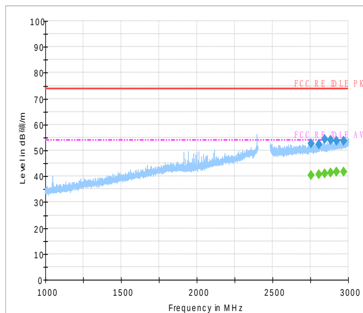
Fig.34 Radiated Spurious Emission (802.11b,Ch1,1GHz~3GHz)
