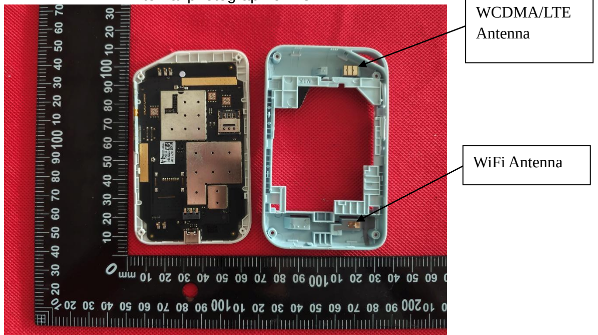
Internal photograph of EUT
