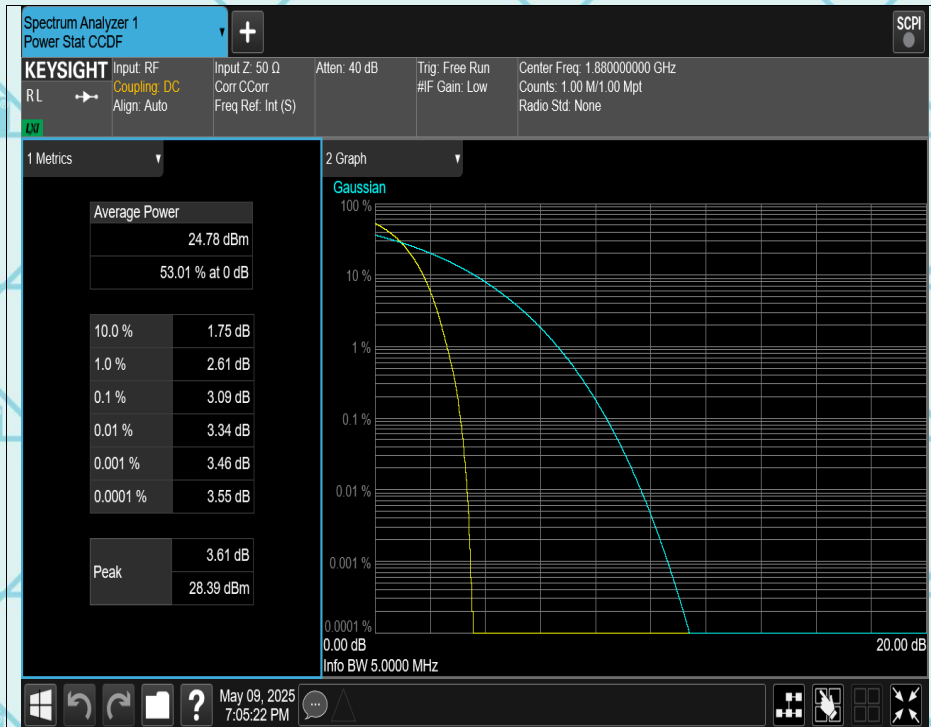
WCDMA Band2 Channel=9400
