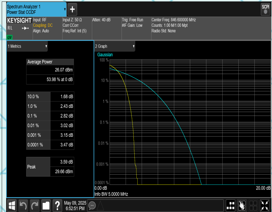
WCDMA Band5 Channel=4233
