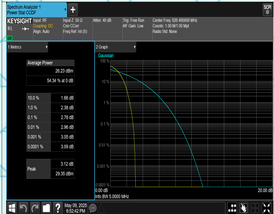
WCDMA Band5 Channel=4132
