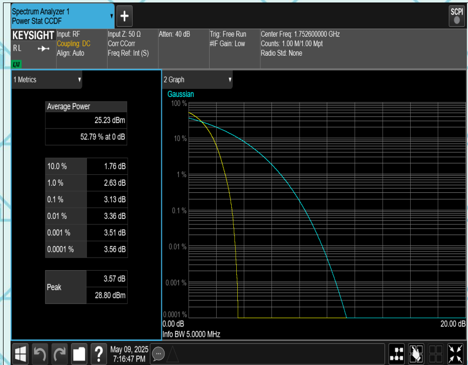
WCDMA Band4 Channel=1513
