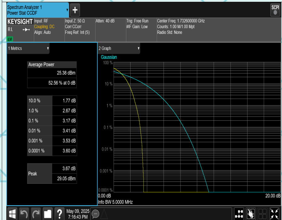
WCDMA Band4 Channel=1413
