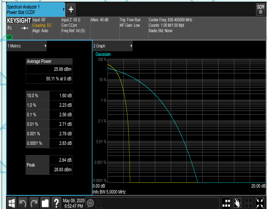
WCDMA Band5 Channel=4182
