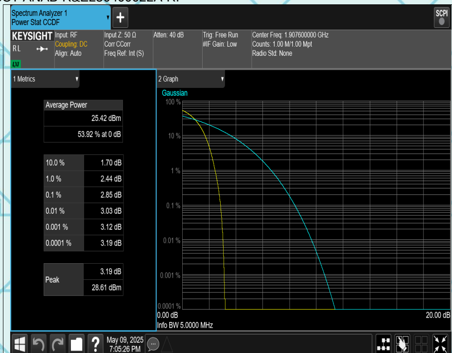
WCDMA Band2 Channel=9538
