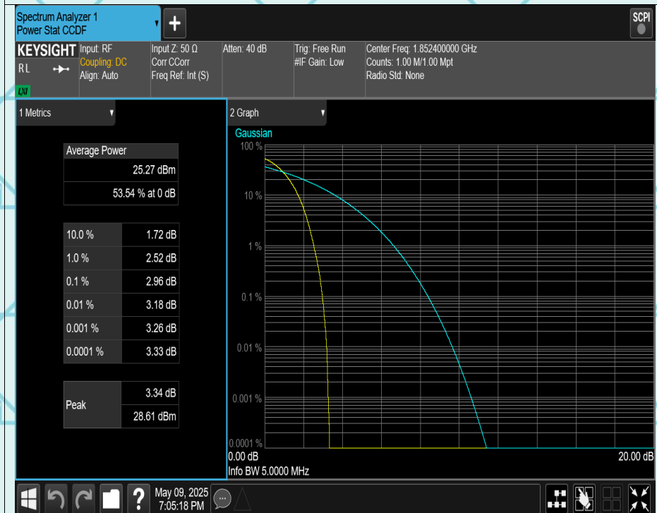
WCDMA Band2 Channel=9262
