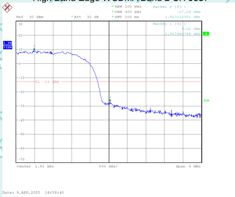
High Band Edge WCDMA Band 2 CH 9537
