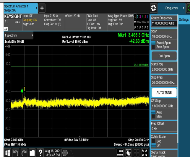
Band4-1.4MHz-16QAM-20175-6RB#0-Range3:2000~20000MHz
