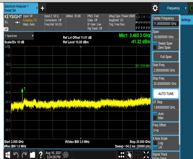
Band4-1.4MHz-QPSK-20175-6RB#0-Range3:2000~20000MHz
