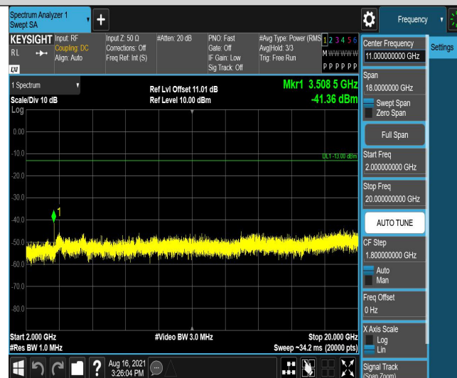
Band4-1.4MHz-16QAM-20393-6RB#0-Range3:2000~20000MHz
