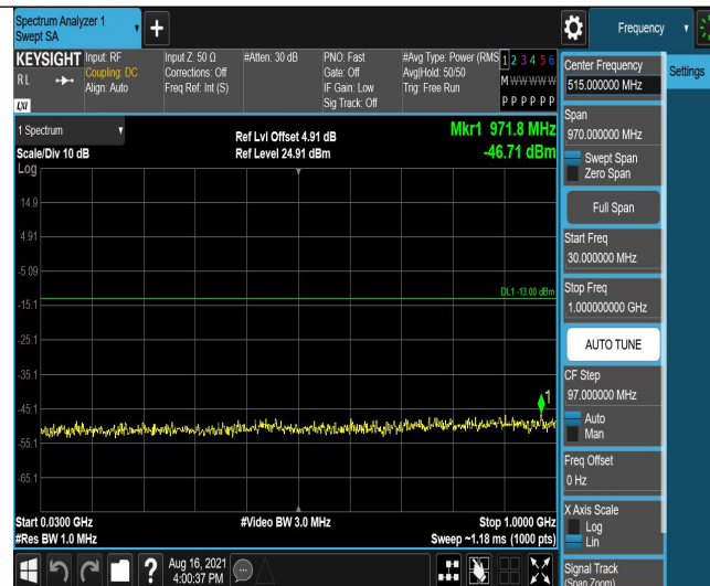
Band4-5MHz-QPSK-19975-25RB#0-Range1:30~1000MHz
