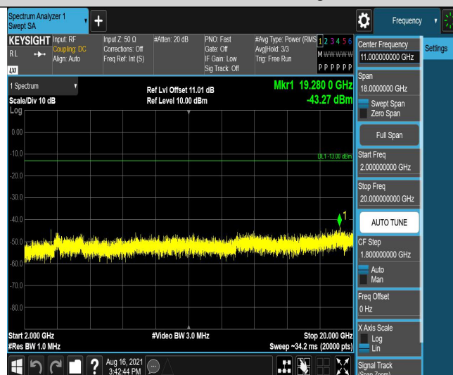
Band4-3MHz-QPSK-20175-6RB#0-Range3:2000~20000MHz
