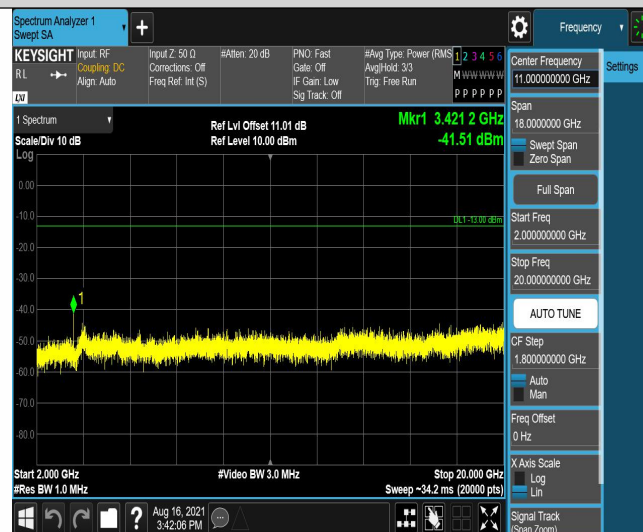
Band4-3MHz-16QAM-19965-6RB#0-Range3:2000~20000MHz
