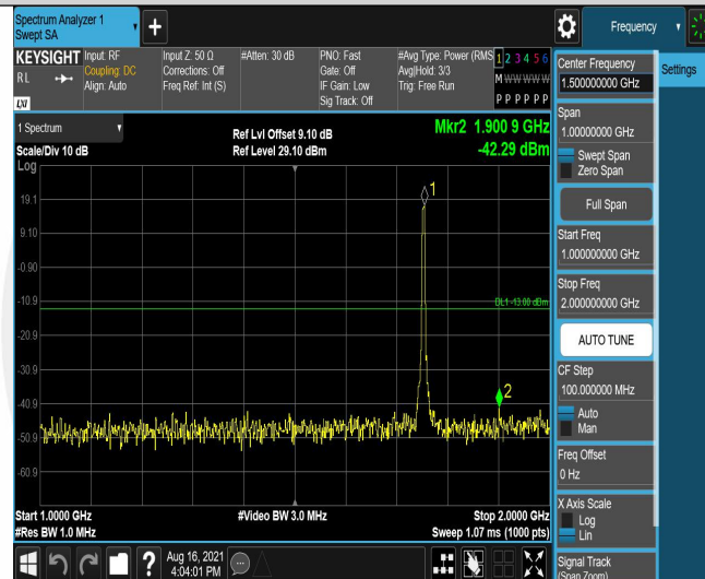
Band4-5MHz-16QAM-20375-25RB#0-Range2:1000~2000MHz
