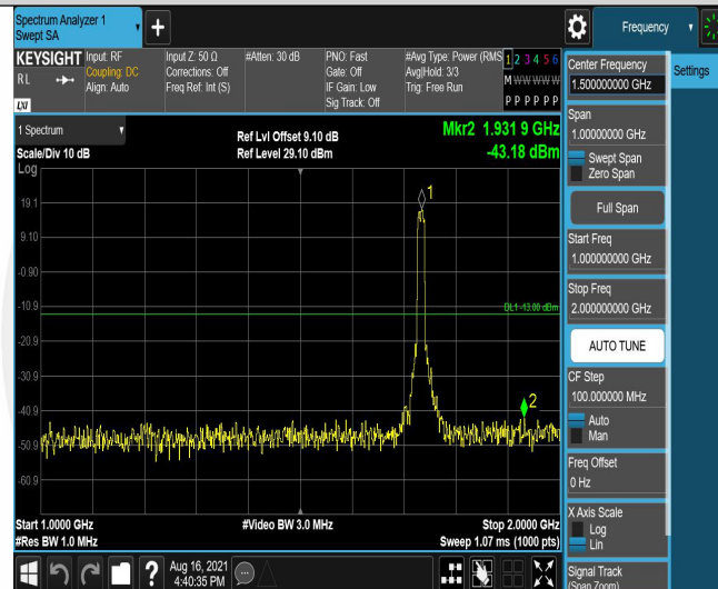
Band4-15MHz-QPSK-20175-75RB#0-Range2:1000~2000MHz
