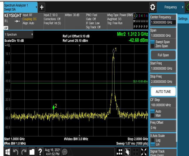
Band4-15MHz-QPSK-20325-75RB#0-Range2:1000~2000MHz
