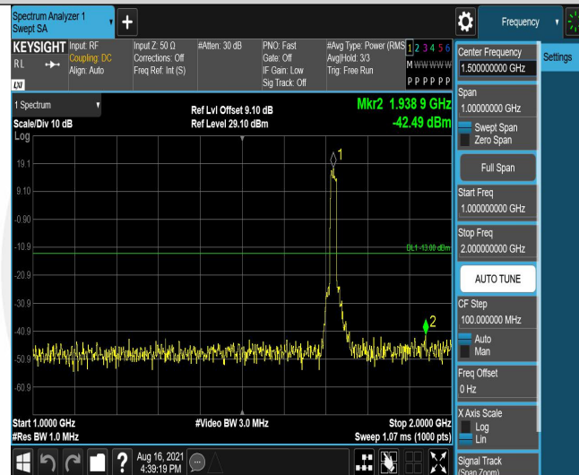
Band4-15MHz-QPSK-20025-75RB#0-Range2:1000~2000MHz
