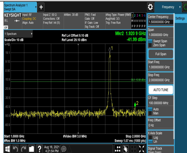
Band4-10MHz-16QAM-20175-50RB#0-Range2:1000~2000MHz
