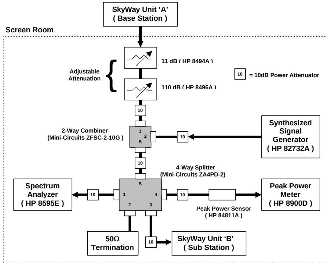
Figure 2 – Equipment Setup
