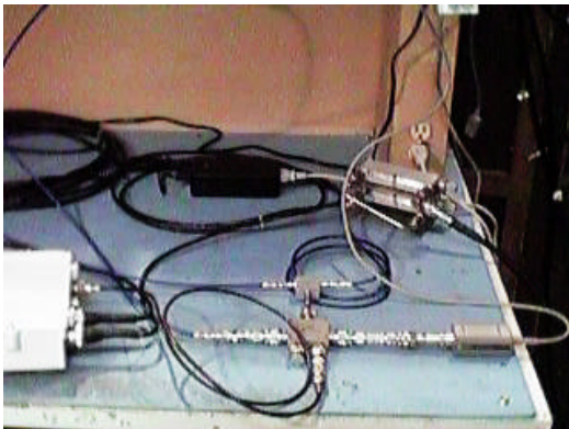
Figure 5 - Setup of attenuators, splitter, and combiner
