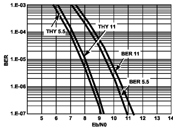
Figure 1 - BER vs. E_b/N_0 Performance for MBOK/CCK Modulation
