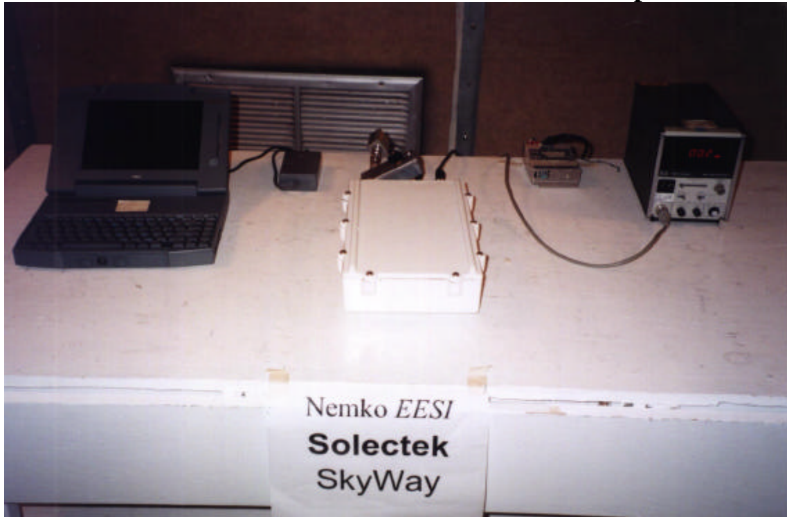
Transmitter Base Station, Fanout Box, Attenuator Pad, Sensor and Peak Power Meter
