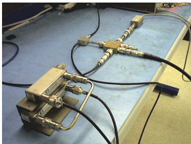
Figure 5 Setup of attenuators, Splitter, and combiner.
