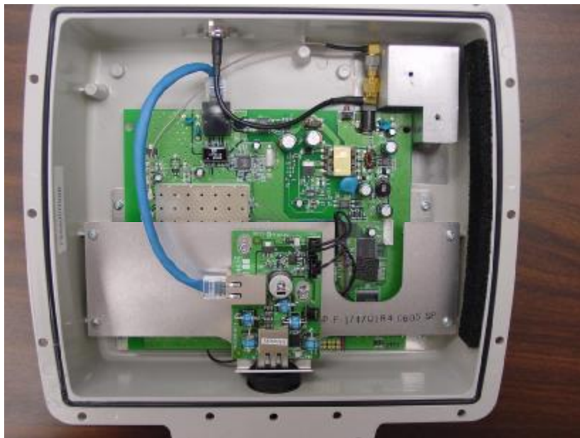
Photo 2: Assembly 2
