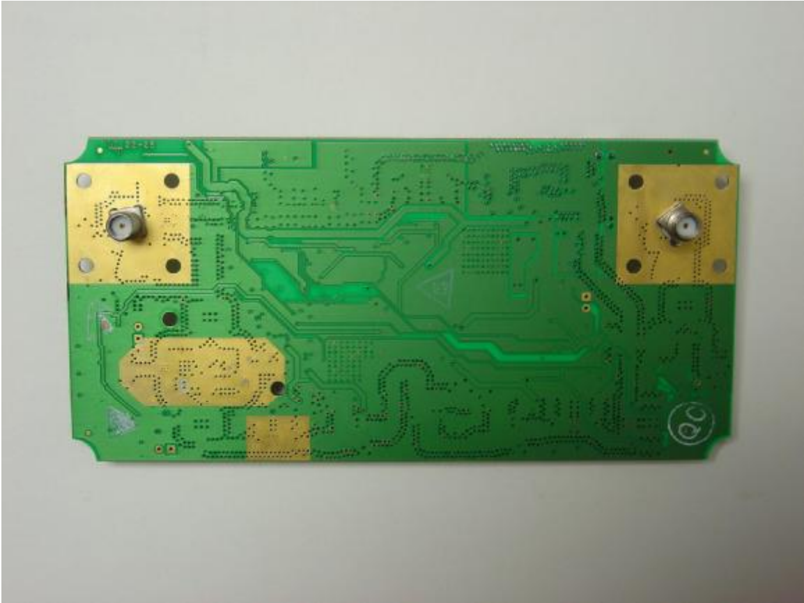
Photo 7: PCB2 bottom
