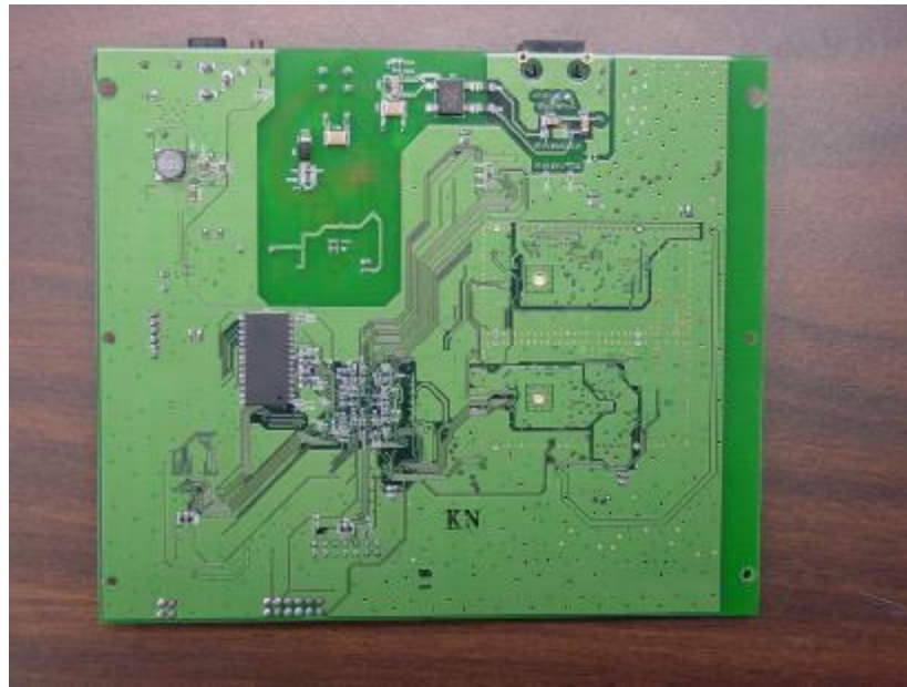
Photo 5: PCB1 bottom
