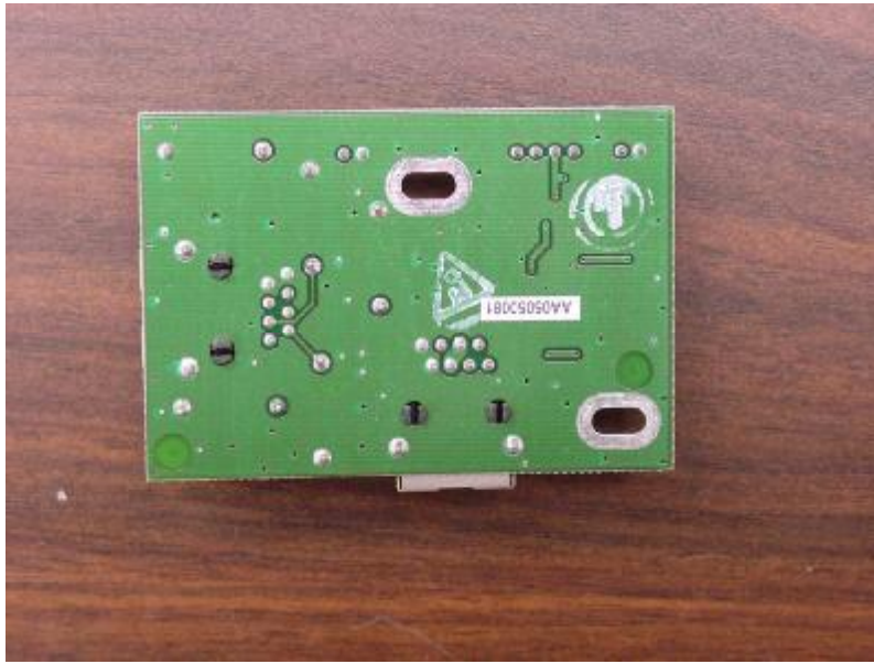
Photo 9: PCB3 bottom
