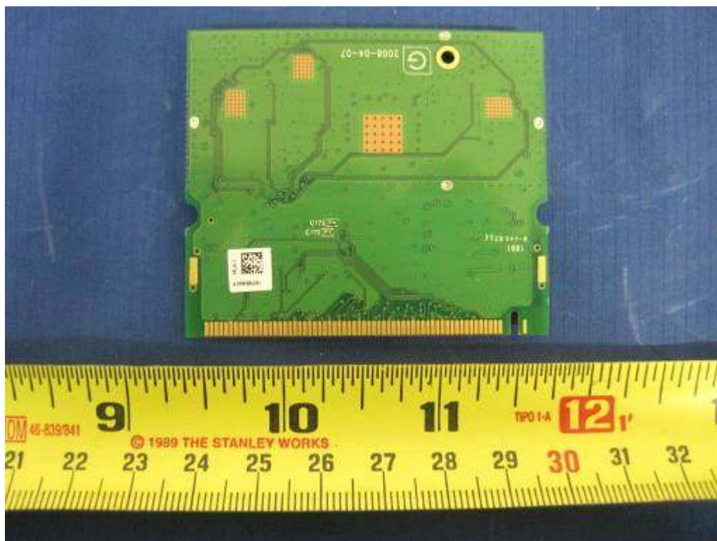
Radio Board – Bottom
