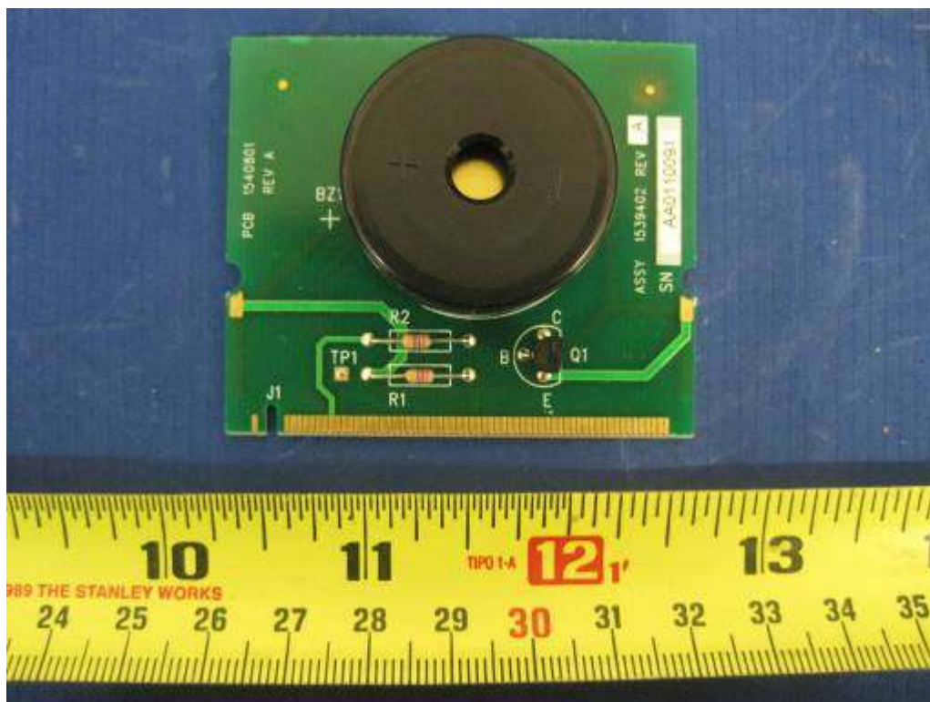
Board A – Top
