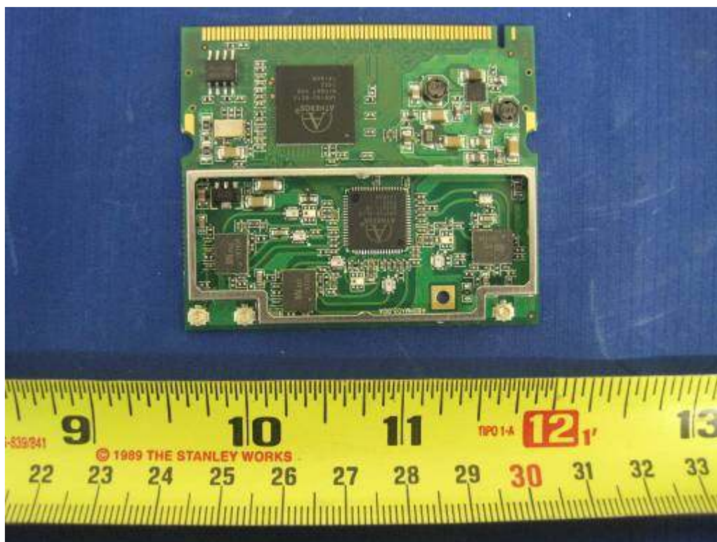
Radio Board – Top (without RF shield)
