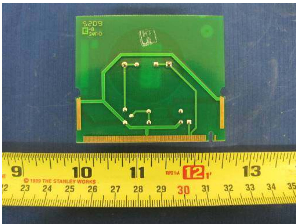
Board A – Bottom
