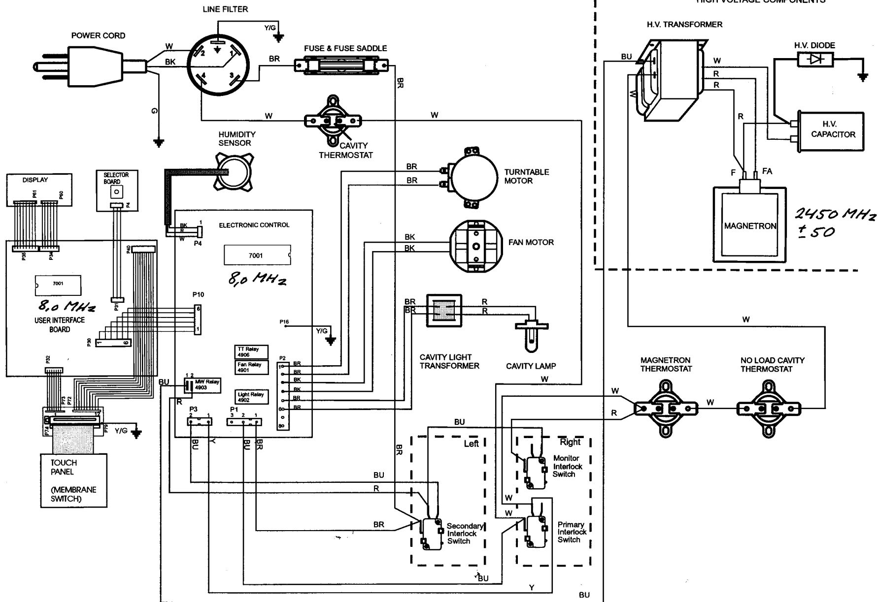
Pictorial Diagram
