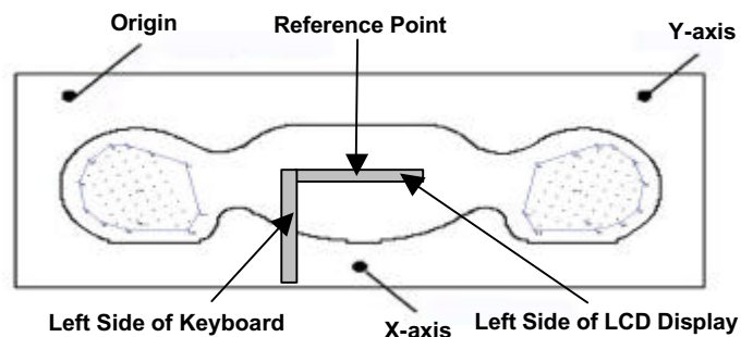
Figure 5. Phantom Reference Point & EUT Positioning Left Side of Laptop PC LCD Display (Open) - Left-Side Antenna
