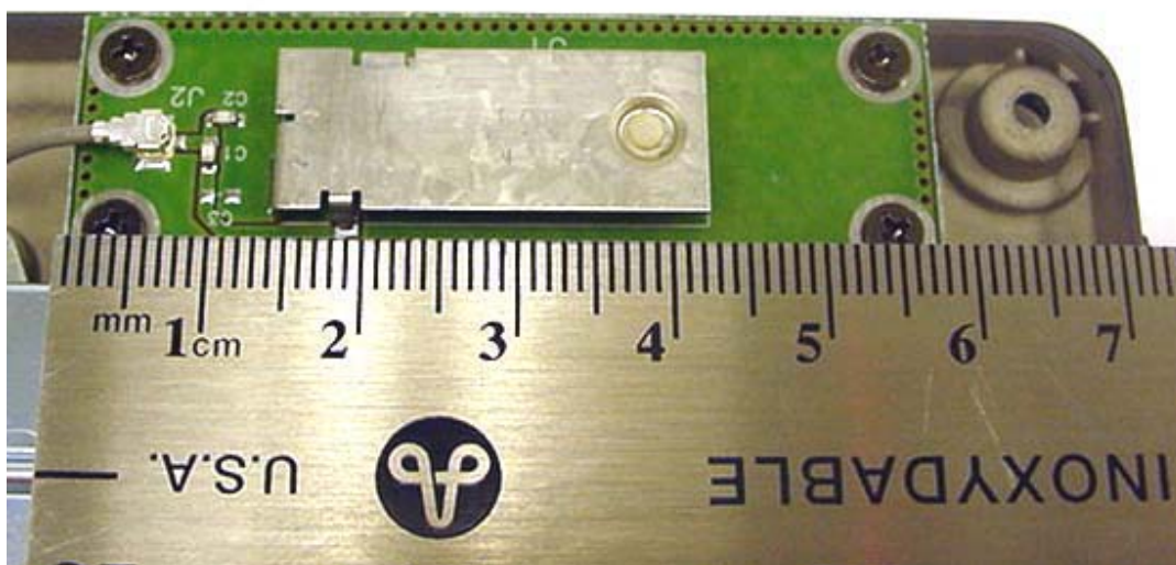
Distance at LCD back-side between dipole antenna feed/swivel-joint and Bluetooth left-side antenna
