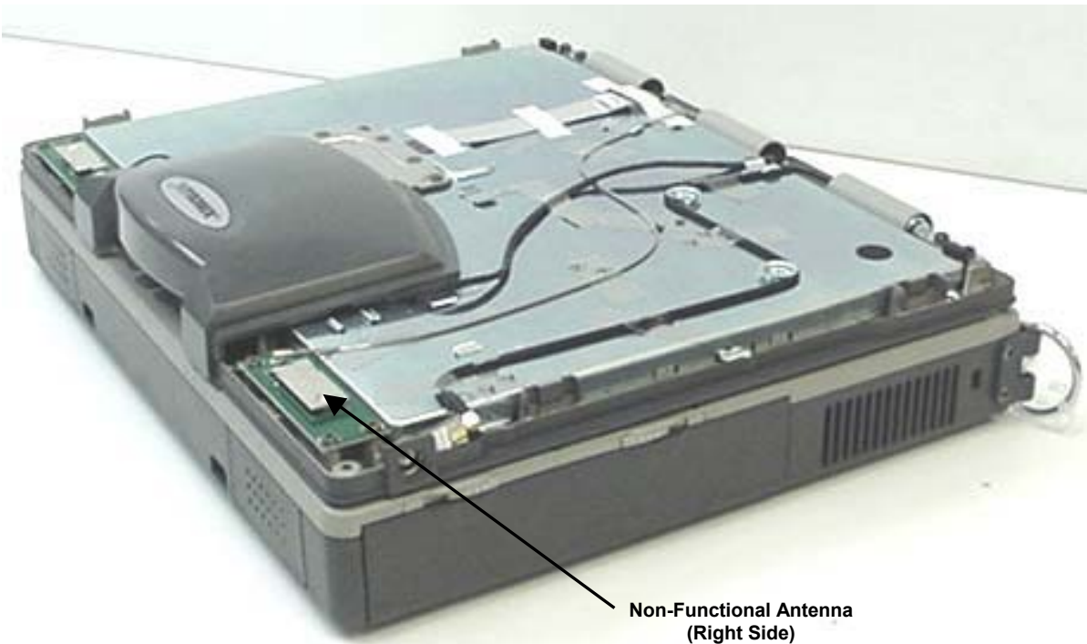
Bluetooth Surface-Mount Antenna (Upper Rear Left Side Edge of LCD Display)
