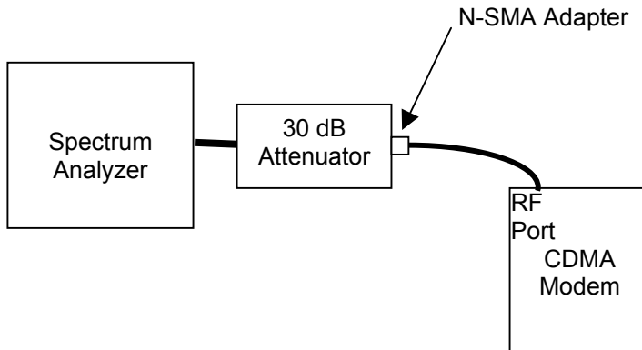
Figure I.6-1 - Setup Drawing
