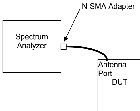
Figure I.6-1 - Setup Drawing
