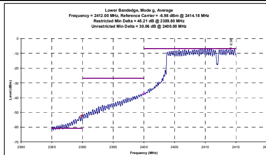
Channel 1 Mode g - Conducted Average Band-edge Plots
