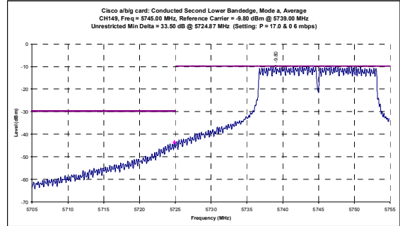
Channel 149 Mode a - Conducted Average Band-edge Plots
