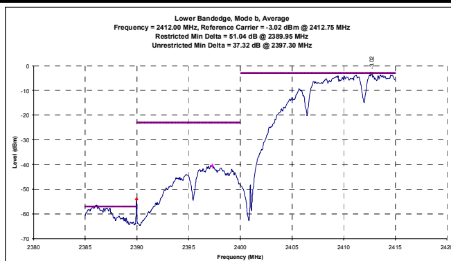
Channel 1 Mode b - Conducted Average Band-edge Plots
