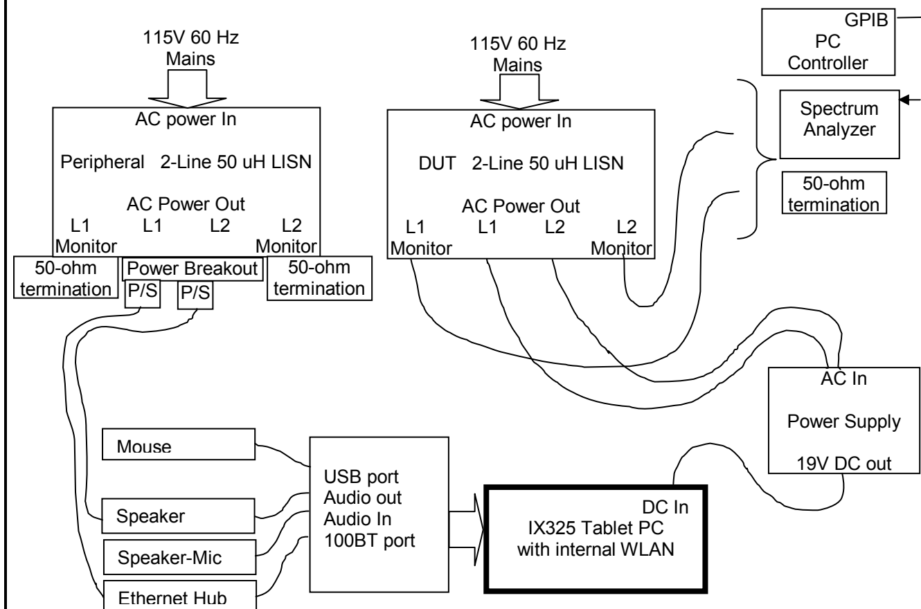
Figure I.6-1 - Setup Drawing
