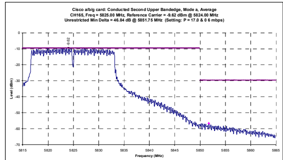
Channel 165 Mode a - Conducted Average Band-edge Plots
