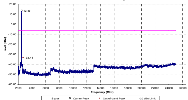
Transmitting Conducted Spurs with 1 MHz RBW & VBW Frequency = 2462 MHz Mode b (1 mbps), Carrier Peak Power = 13.46 dBm Maximum Out-of-Band Emission = -33.41dBm @ 2688.00 MHz
