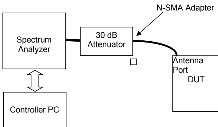
Figure H.6-1 - Setup Drawing
