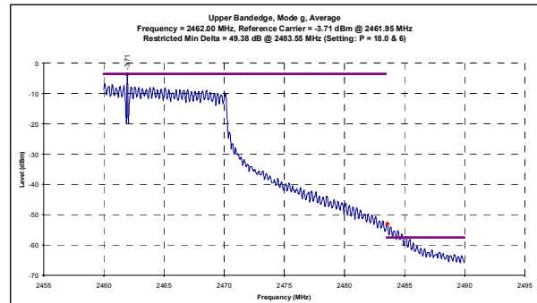
Channel 11 Mode g - Conducted Average Band-edge Plots
