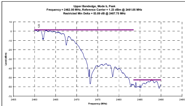
Channel 11 Mode b - Conducted Peak Band-edge Plots
