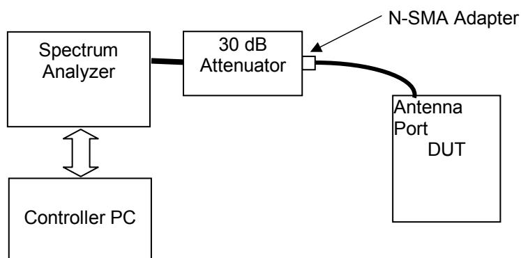
Figure E.6-1 - Setup Drawing
