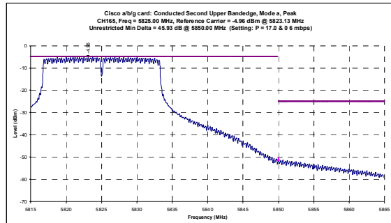
Channel 165 Mode a - Conducted Peak Band-edge Plots
