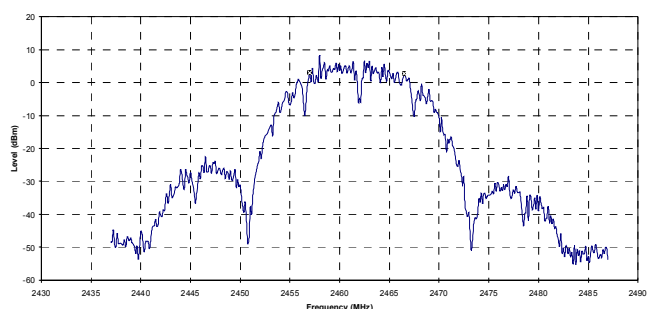
IX325 with Cisco abg WLAN Settings: 20.0 & 0.1 mbps, Frequency = 2462 MHz, Mode b, -6 dB Emission Bandwidth = 9.50 MHz with an RBW of 100 kHz
