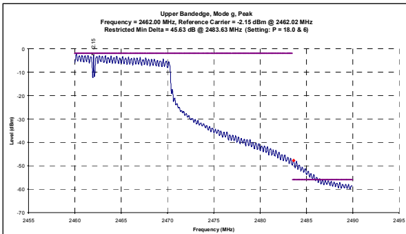
Channel 11 Mode g - Conducted Peak Band-edge Plots
