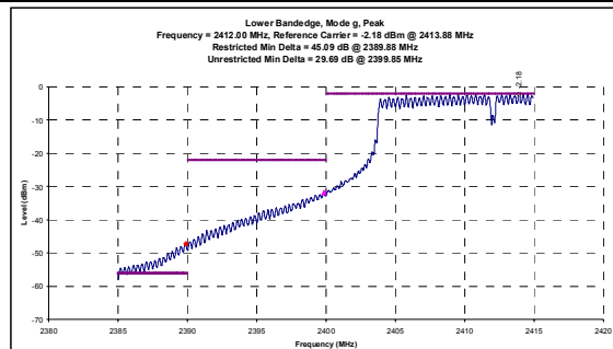
Channel 1 Mode g - Conducted Peak Band-edge Plots
