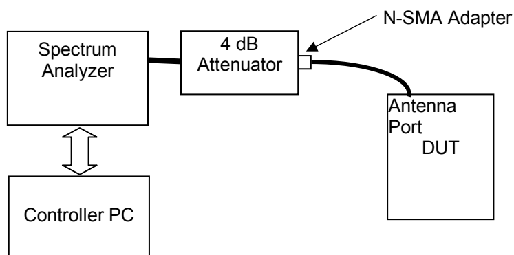
Figure D.6-1 - Setup Drawing
