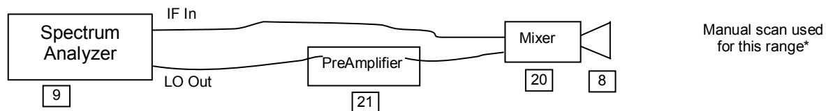
Figure G.6-2 - Setup Drawing ( \geq 26.5 GHz)
