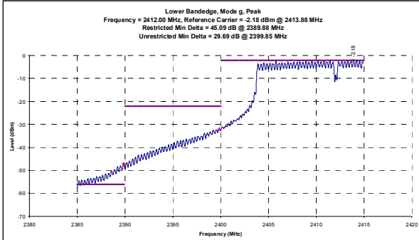
Channel 1 Mode g - Conducted Peak Band-edge Plots
