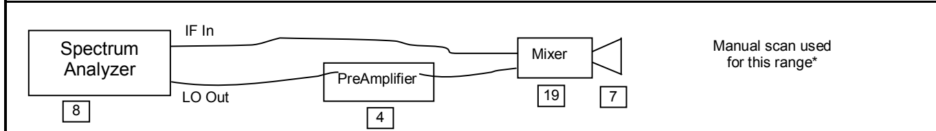
Figure F.6-2 - Setup Drawing ( \geq 26.5 GHz)
