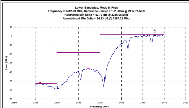
Channel 1 Mode b - Conducted Peak Band-edge Plots
