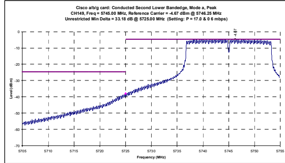
Channel 149 Mode a - Conducted Peak Band-edge Plots
