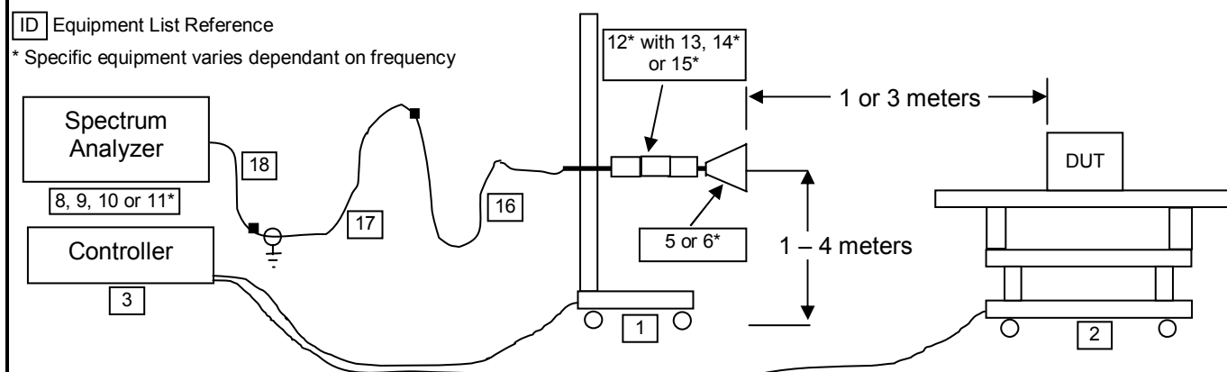
Figure F.6-1 - Setup Drawing ( \leq 26.5 GHz)
