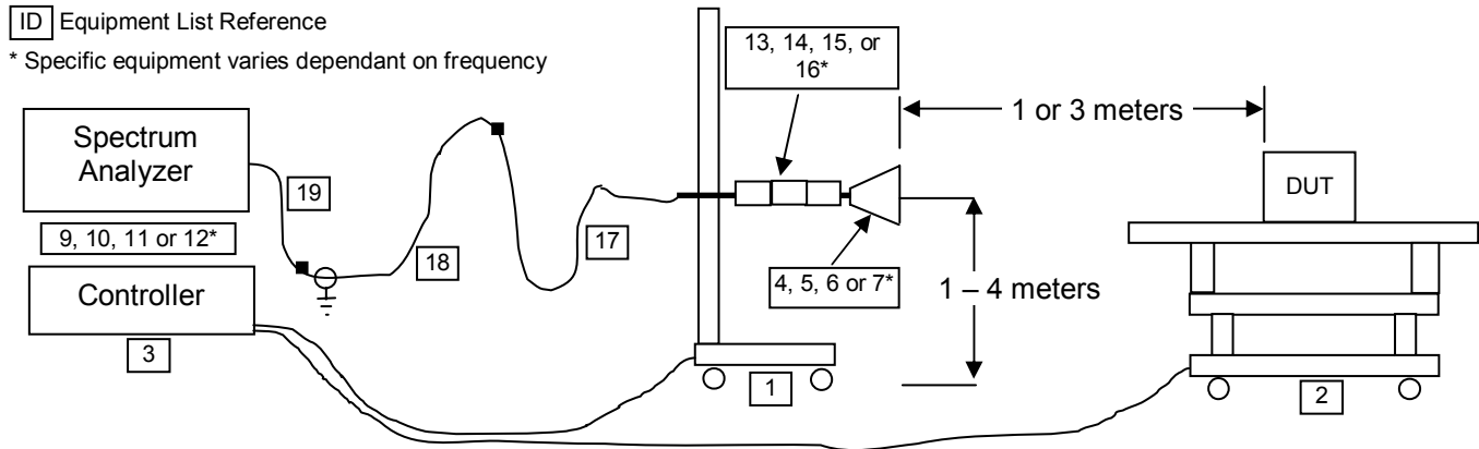
Figure G.6-1 - Setup Drawing ( \leq 26.5 GHz)
