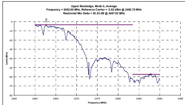
Channel 11 Mode b - Conducted Average Band-edge Plots
