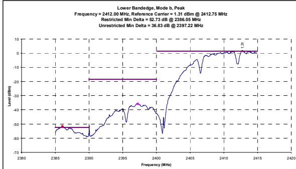
Channel 1 Mode b - Conducted Peak Band-edge Plots
