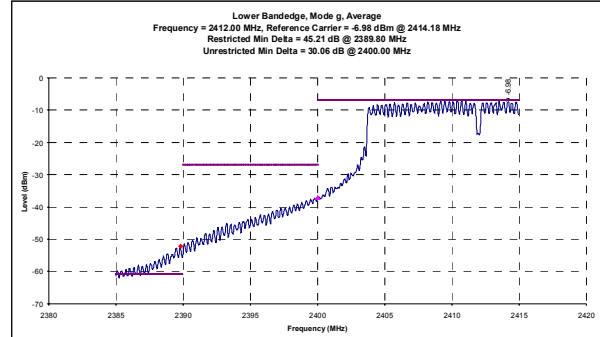
Channel 1 Mode g - Conducted Average Band-edge Plots
