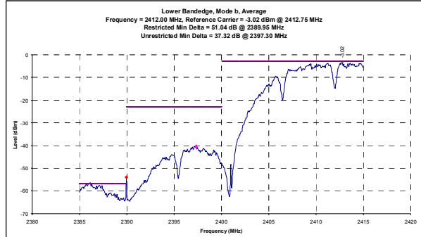
Channel 1 Mode b - Conducted Average Band-edge Plots
