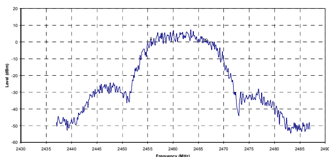
IX325 with Cisco abg WLAN Settings: 20.0 & 0.11 mbps, Frequency = 2462 MHz, Mode b, -6 dB Emission Bandwidth = 11.00 MHz with an RBW of 100 kHz
