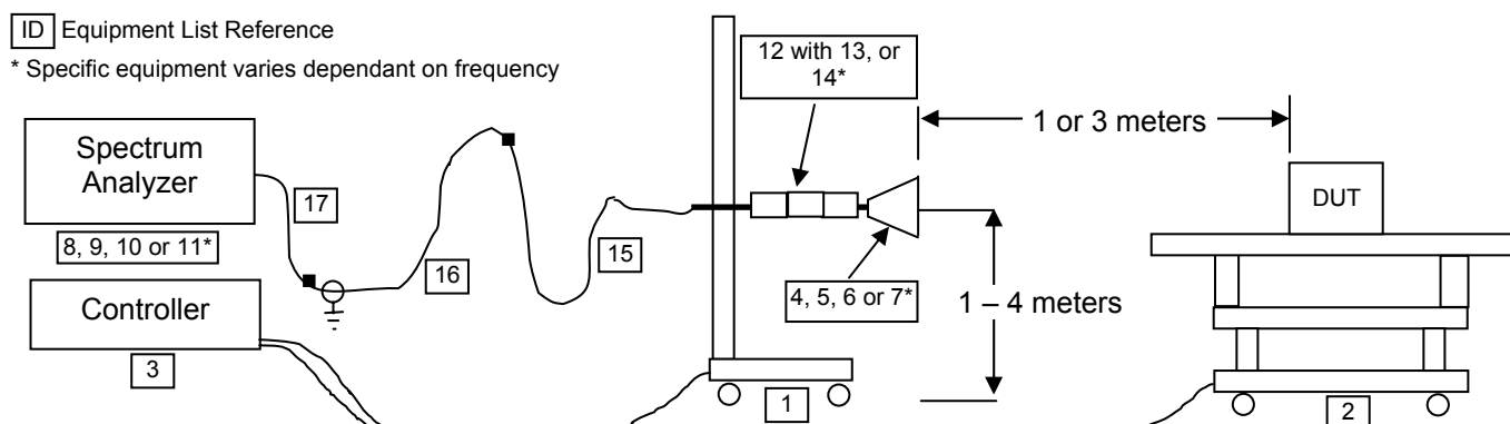
Figure F.6-1 - Setup Drawing
