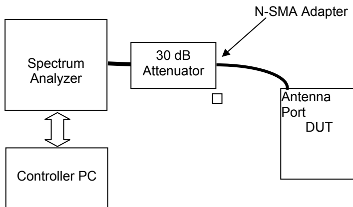
Figure G.6-1 - Setup Drawing
