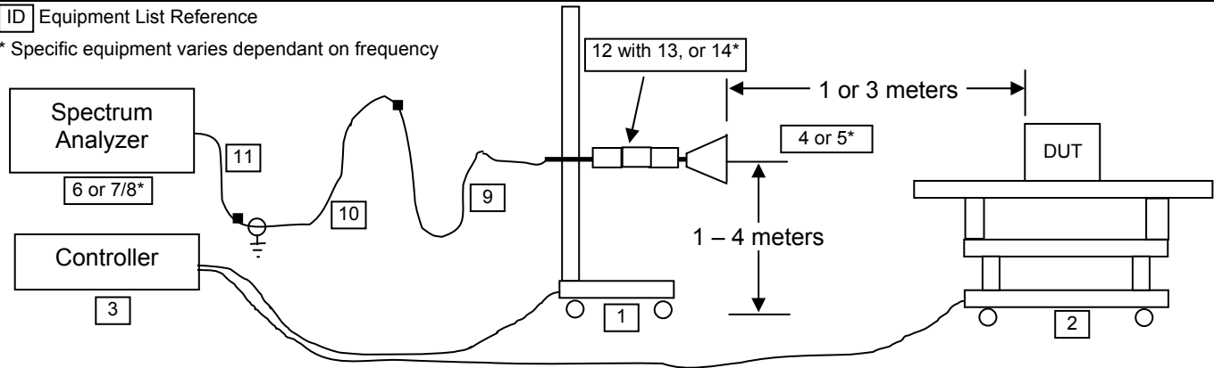
Figure K.6-1 - Field Strength Setup Drawing
