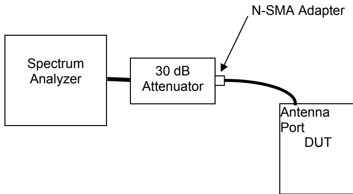
Figure C.6-1 - Setup Drawing
