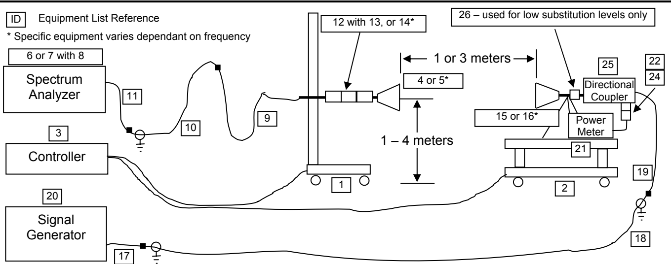
Figure F.6-2 - Signal Substitution Setup Drawing
