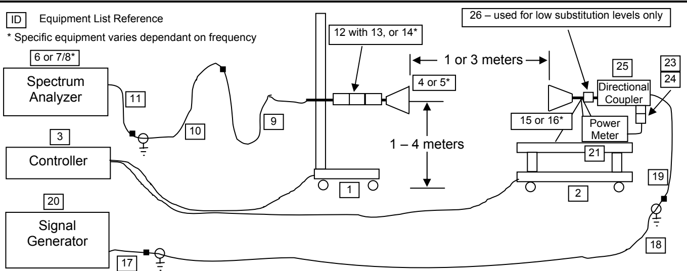
Figure K.6-2 - Signal Substitution Setup Drawing
