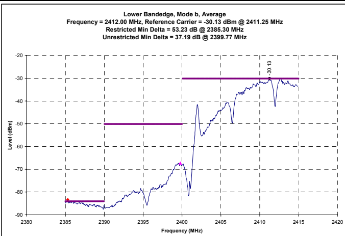
Channel 1 Mode b - Conducted Average Band-edge Plots
