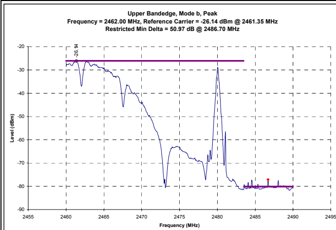
Channel 11 Mode b - Conducted Peak Band-edge Plots
