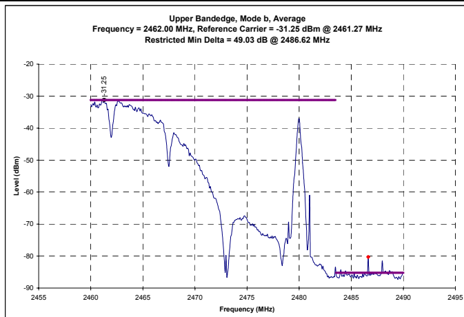
Channel 11 Mode b - Conducted Average Band-edge Plots
