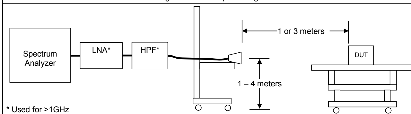
Figure I.6-1 - Setup Drawing
