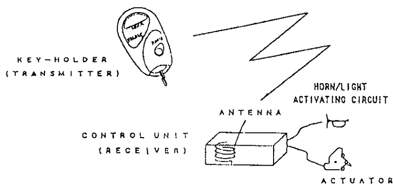
Figure 1-1 : System construction
