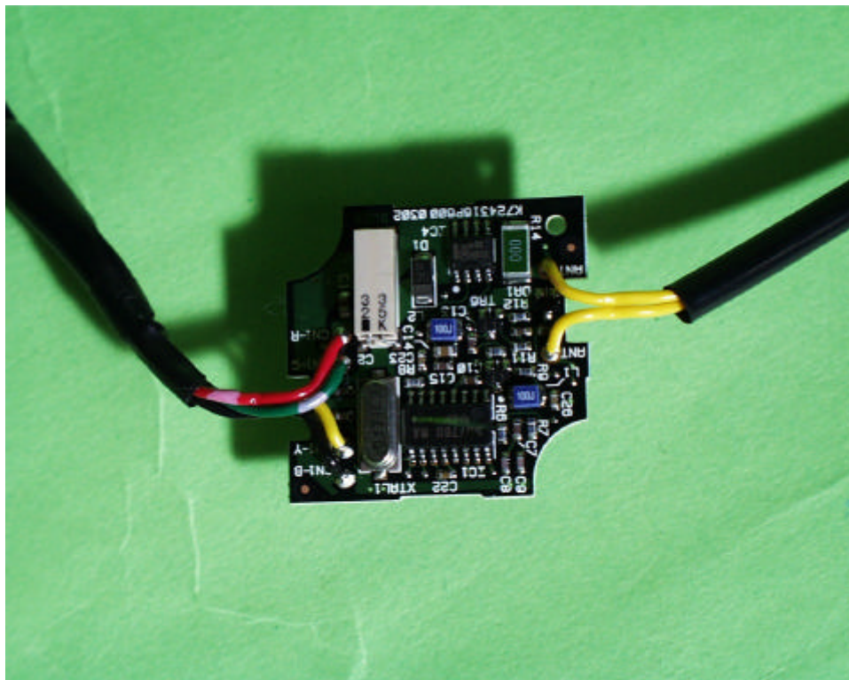
Circuit Board (Back)
