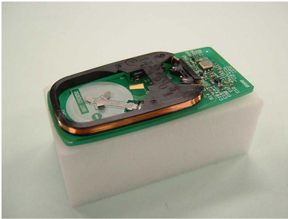
Coil Antenna
