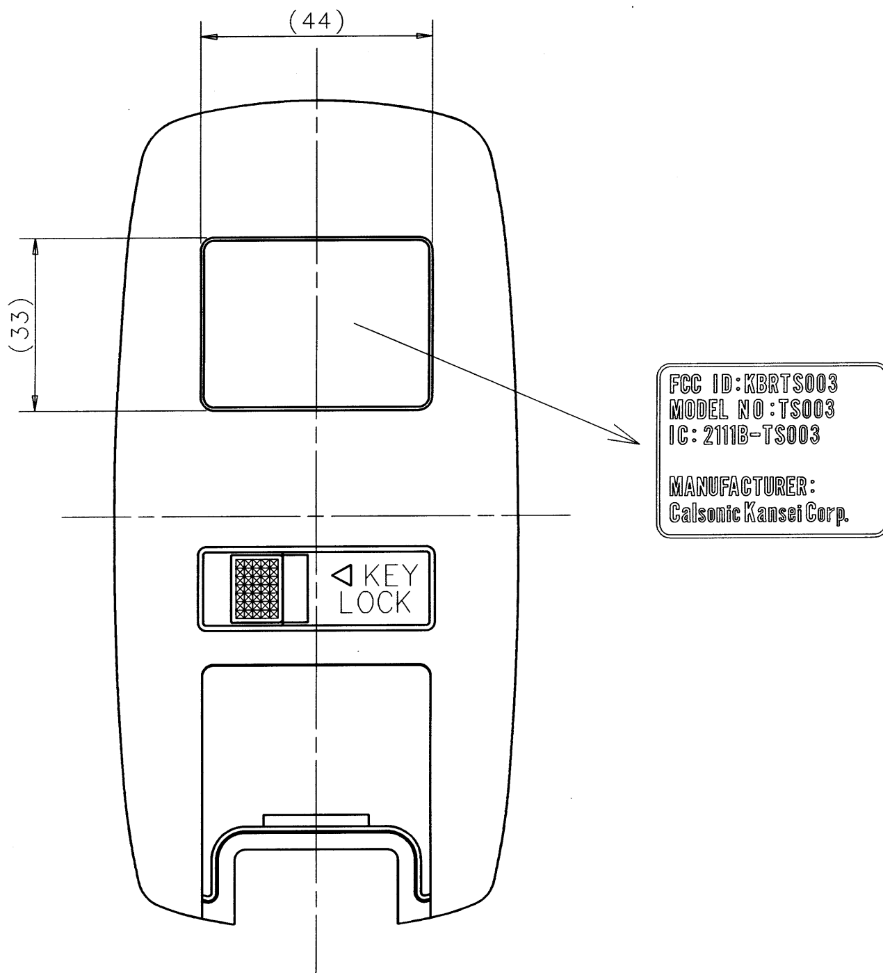
Back surface of transmitter
