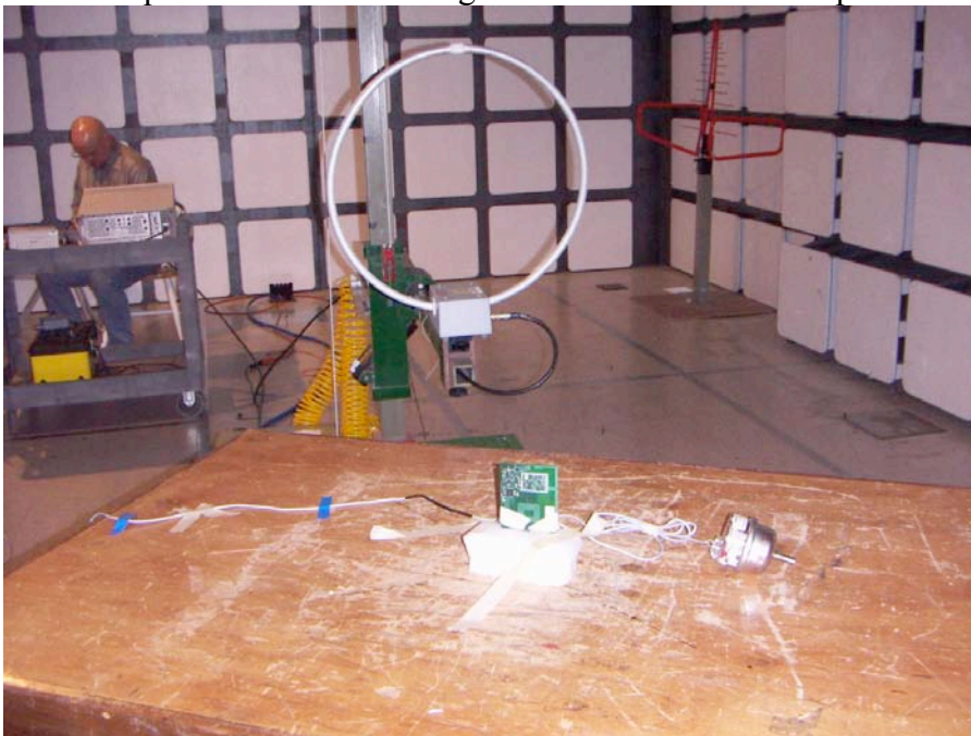
Touchcoupler and Universal Programmer interface test setup
